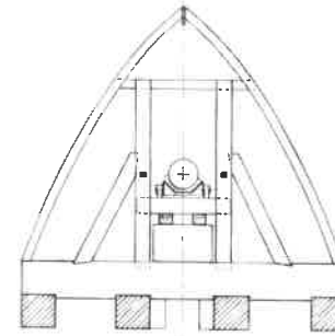
ELEVATION OF HEAD WALL
