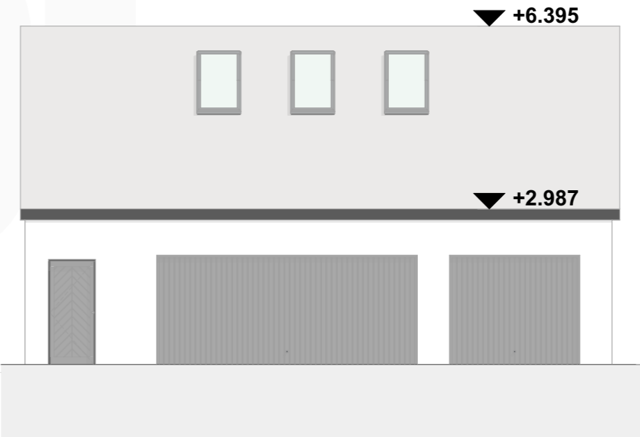
1:100 West Elevation
