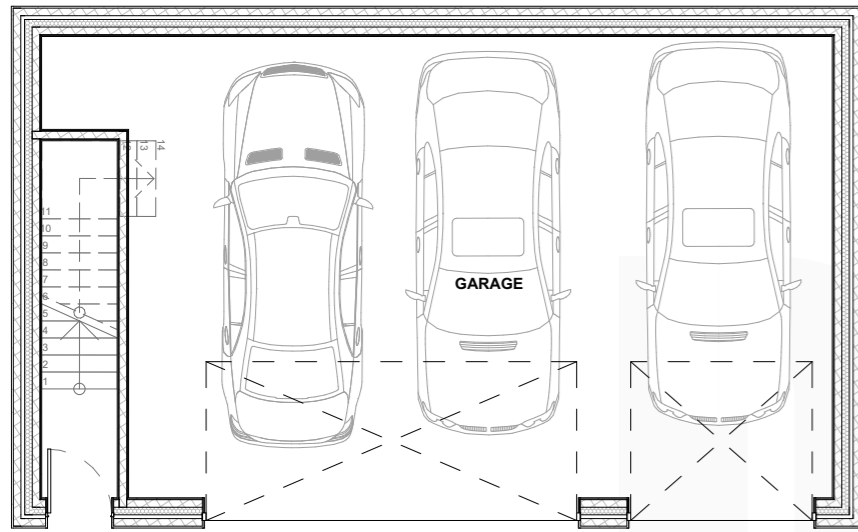
1.100 Ground Floor
