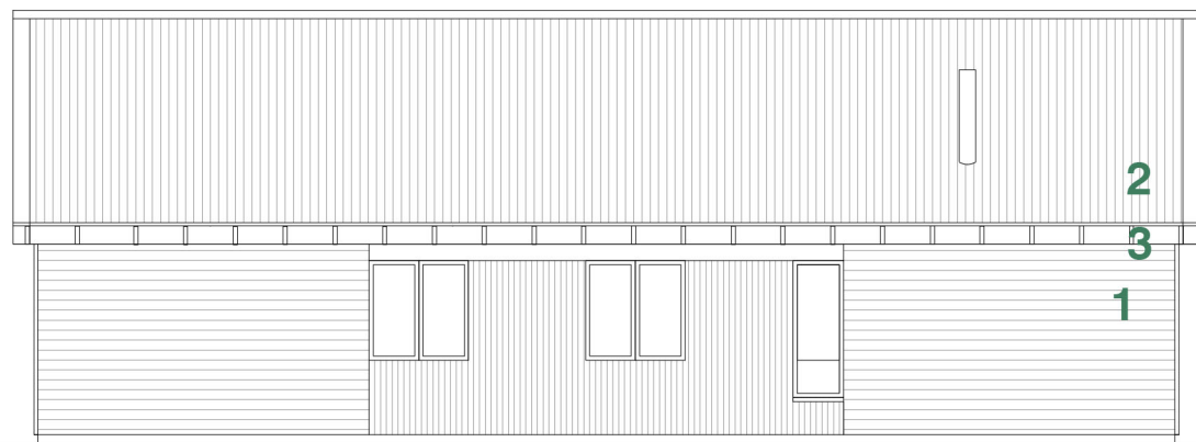
Proposed north elevation Scale 1:100@A3
