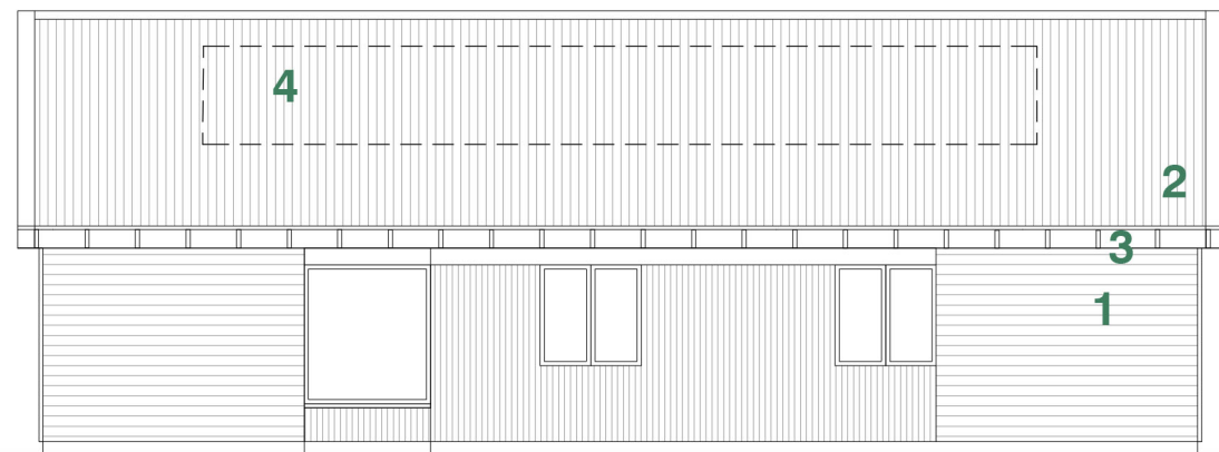
Proposed south elevation Scale 1:100@A3
