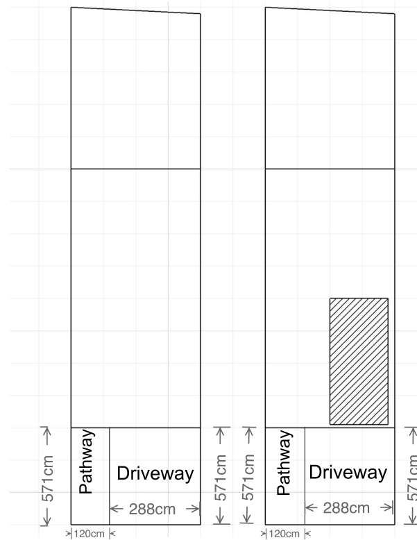
Existing block plan Proposed block plan
