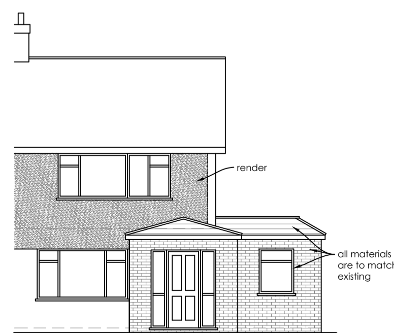
Front elevation 1:100
