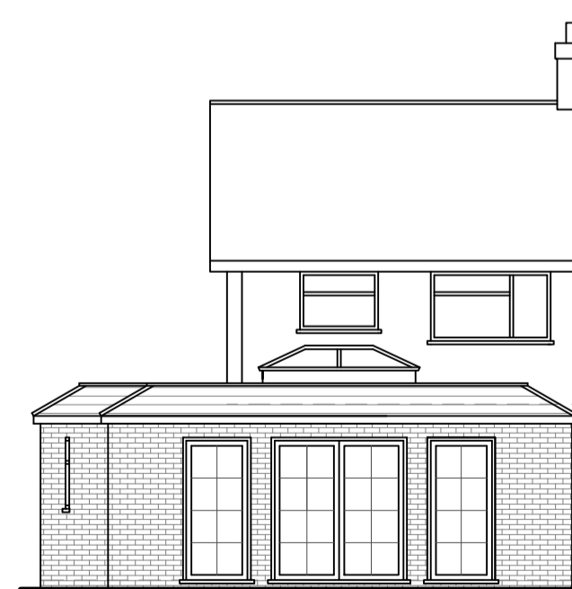
Rear elevation 1:100
