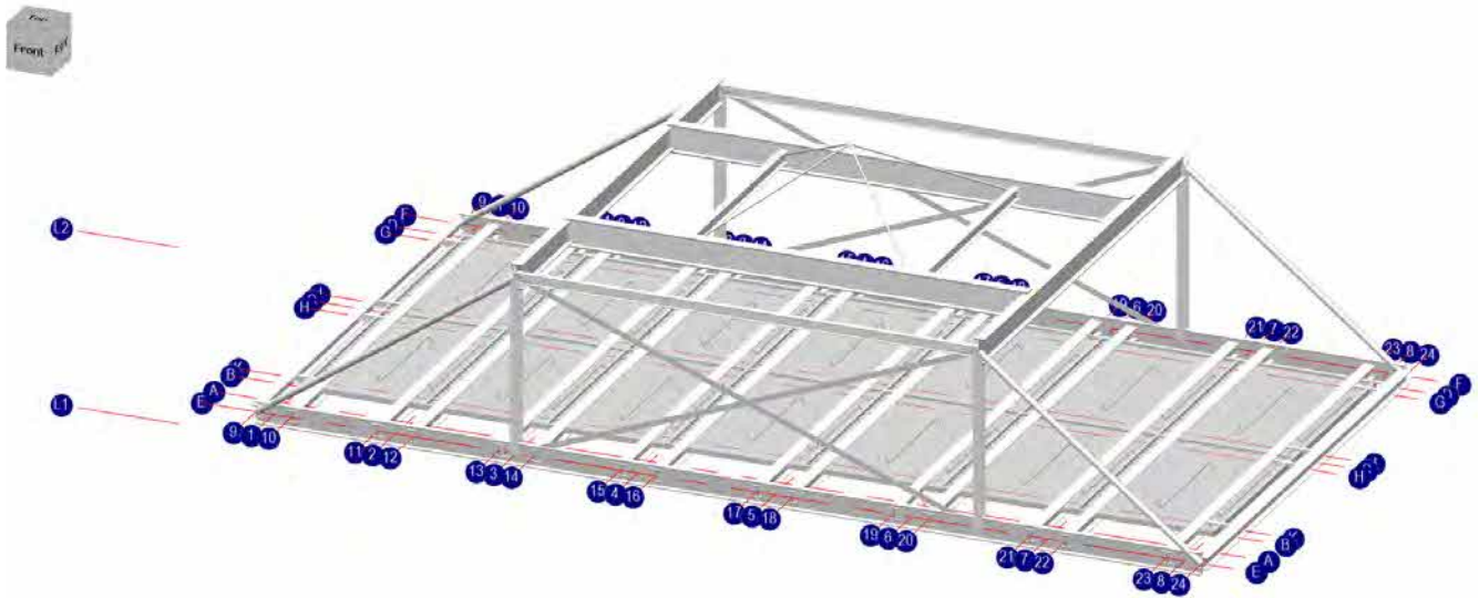
Lifting Frame for Flat Roofed Building
