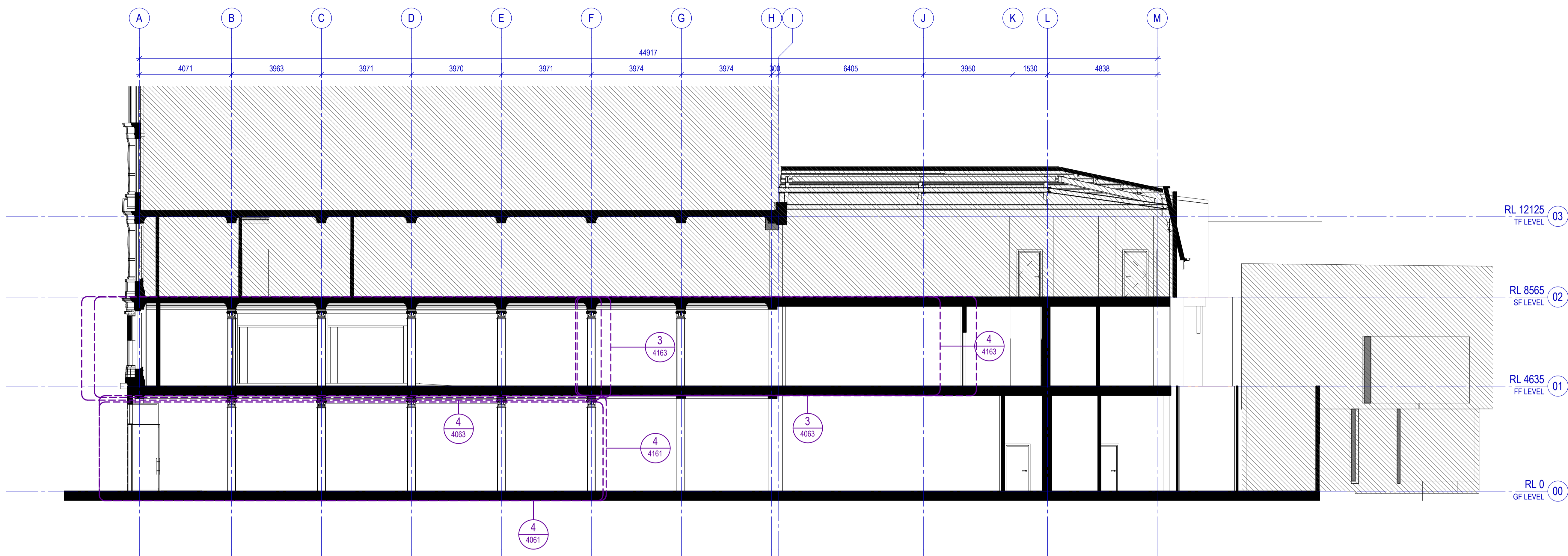
2 Section - North - Existing SCALE 1 : 100
