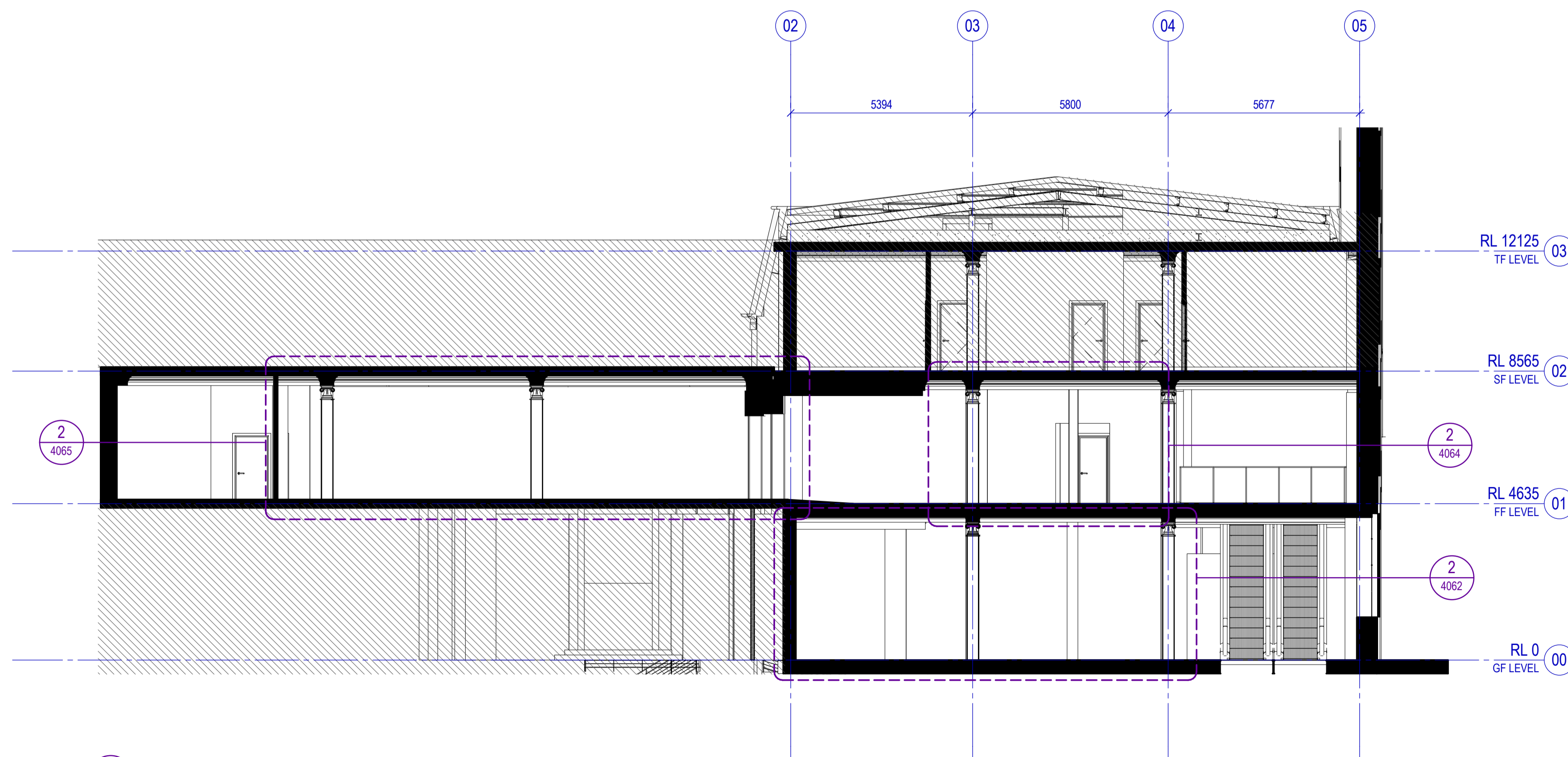
1 Section - East - Existing SCALE 1 : 100
