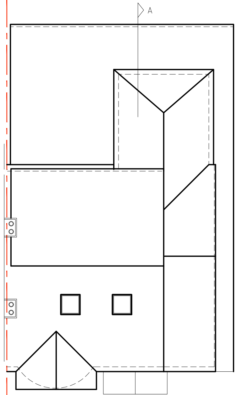
PROPOSED ROOF PLAN 1:100@A3
