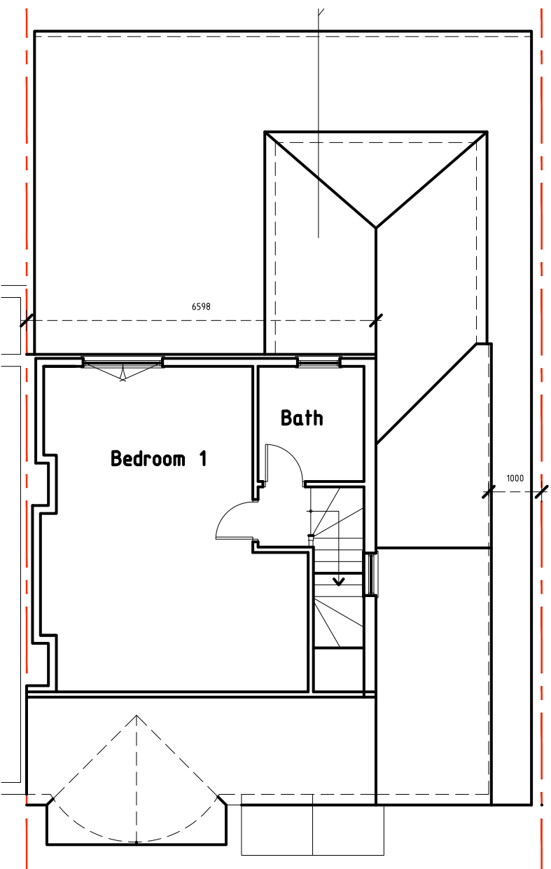
PROPOSED LOFT PLAN 1:100@A3
