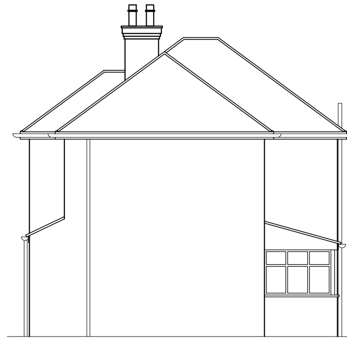
EXISTING SIDE (NORTH-EAST) ELEVATION
