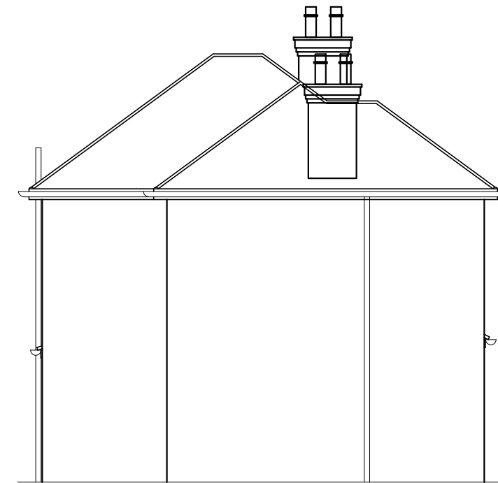
EXISTING SIDE (SOUTH-WEST) ELEVATION
