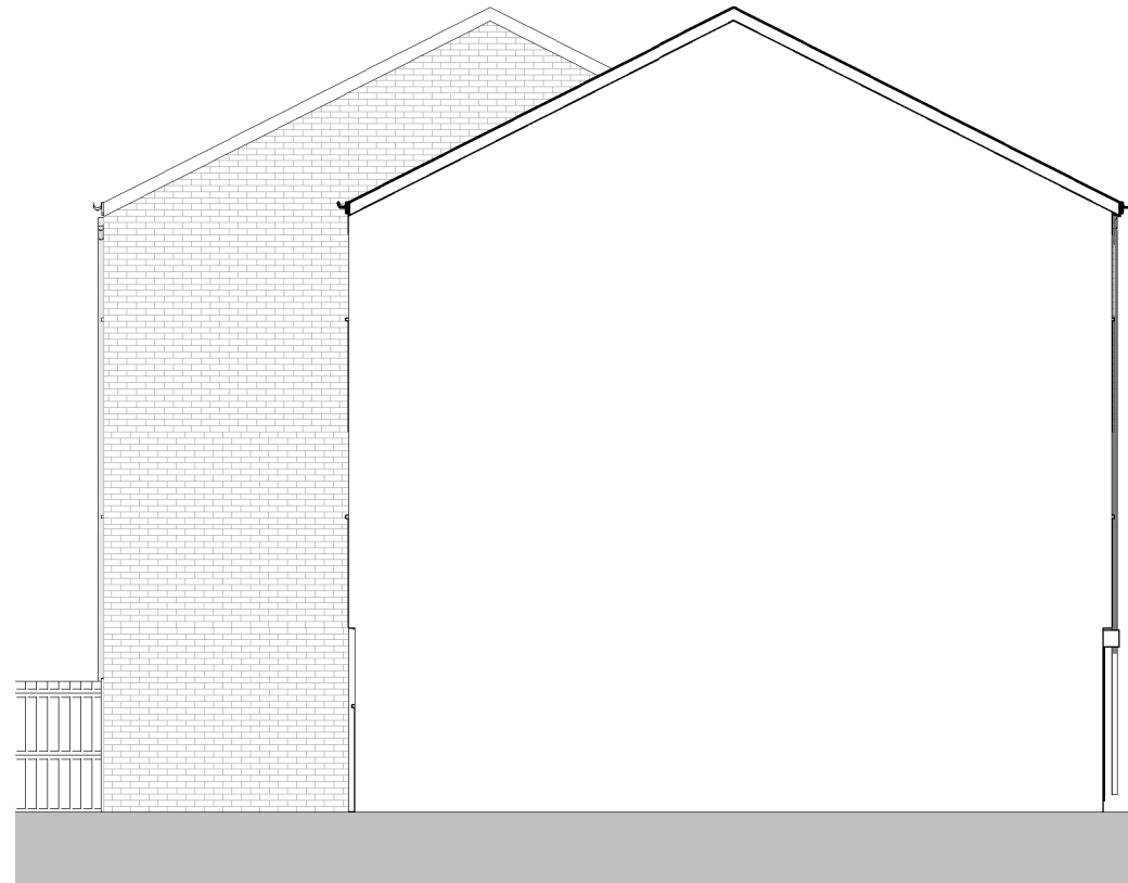
Existing Elevation
