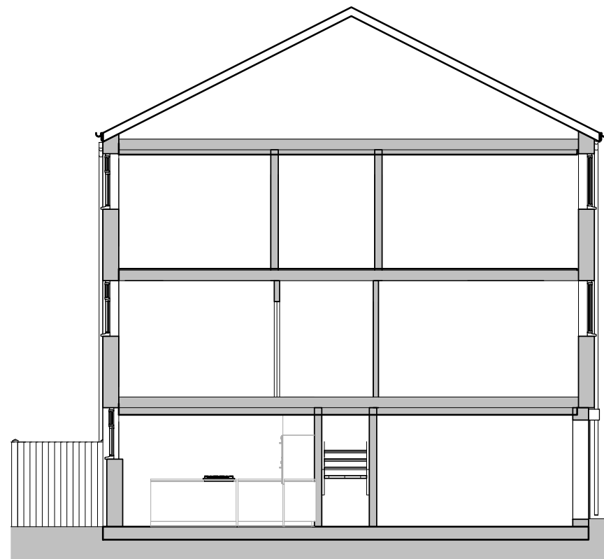
Existing Section
