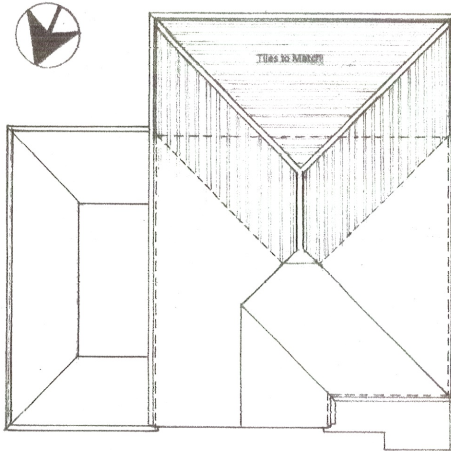
ROOF PLAN
