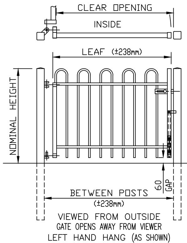
GATE SECURED USING PADLOCKABLE DROPBOLT & SLIDE LATCH
