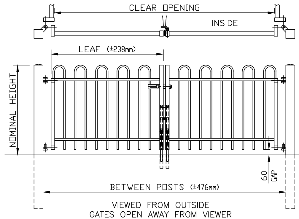
GATES SECURED USING PADLOCKABLE DROPBOLTS & SLIDE LATCH
