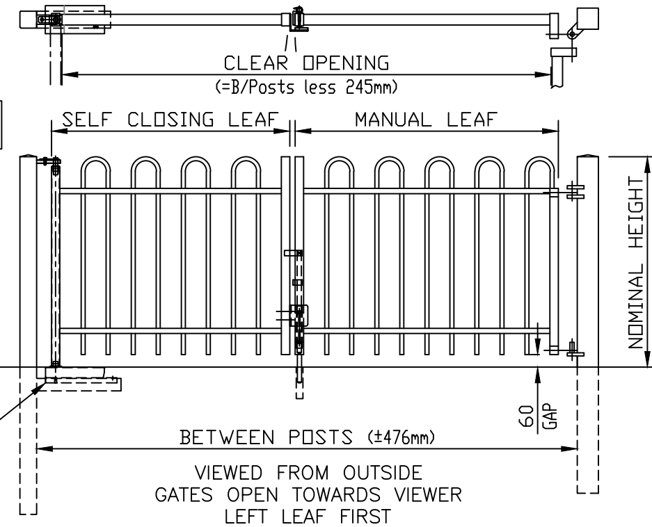
MANUAL LEAF SECURED USING PADLOCKABLE DROPBOLT
