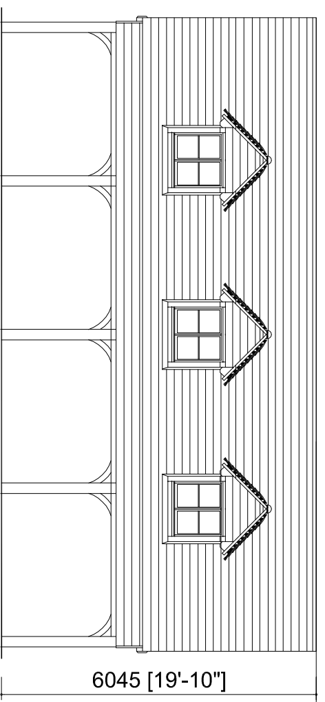
PROPOSED FRONT ELEVATION A SCALE 1:200
