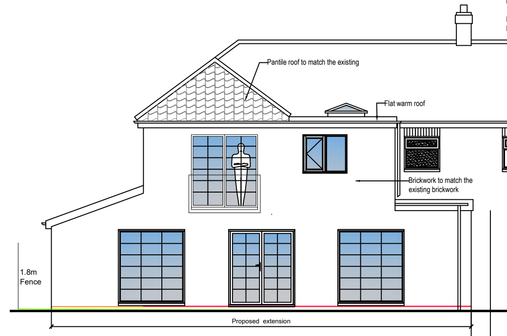
East Elevation 1:100
