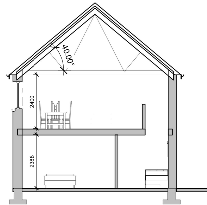
Section thru dining 1 : 100
