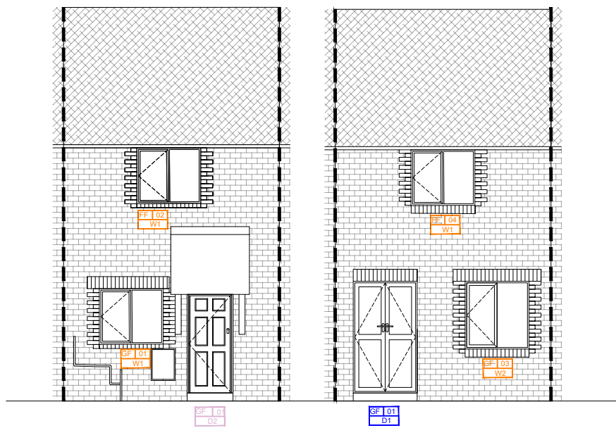
FRONT ELEVATION: 1:100
