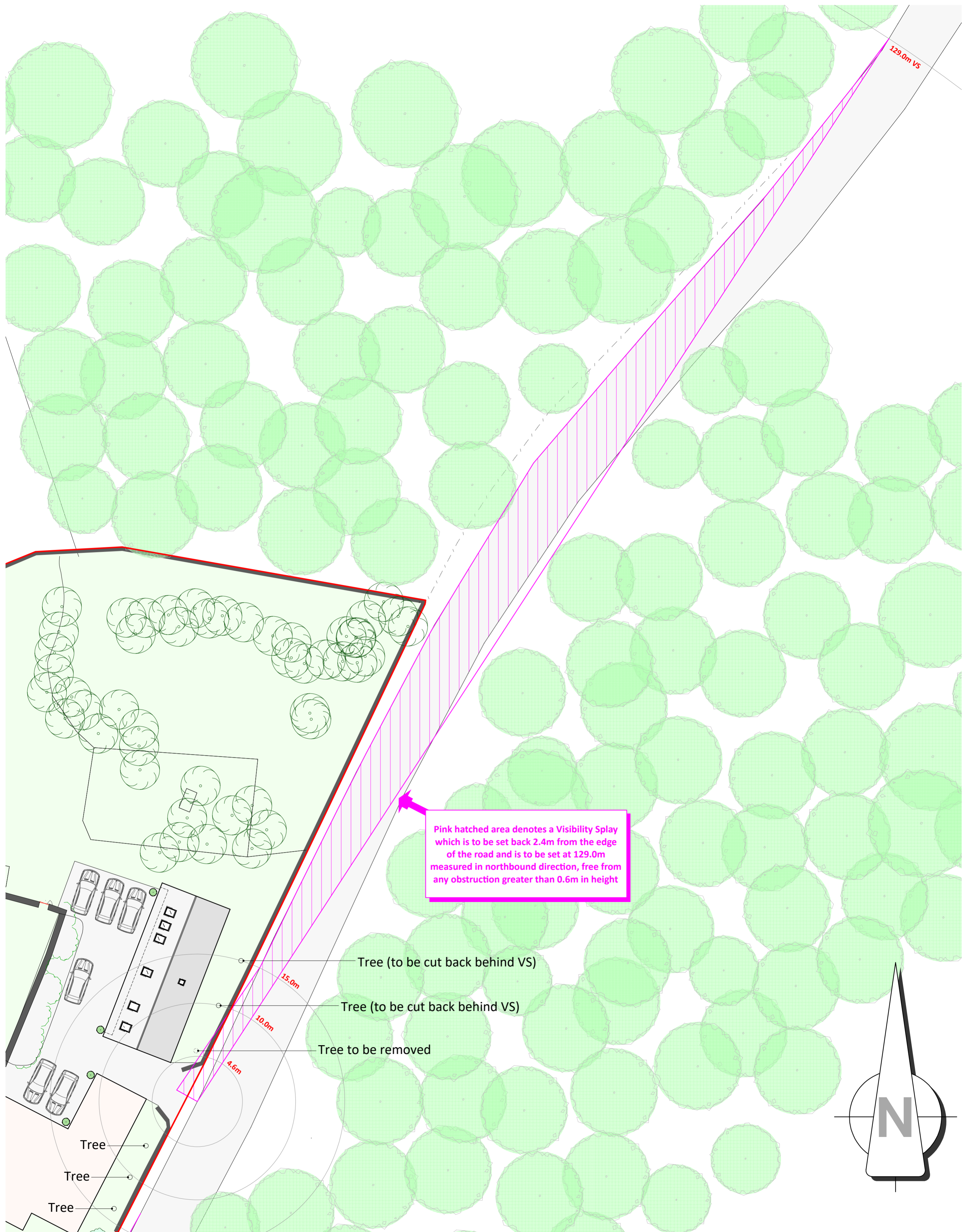
VS Plan (north) - scale 1:250
