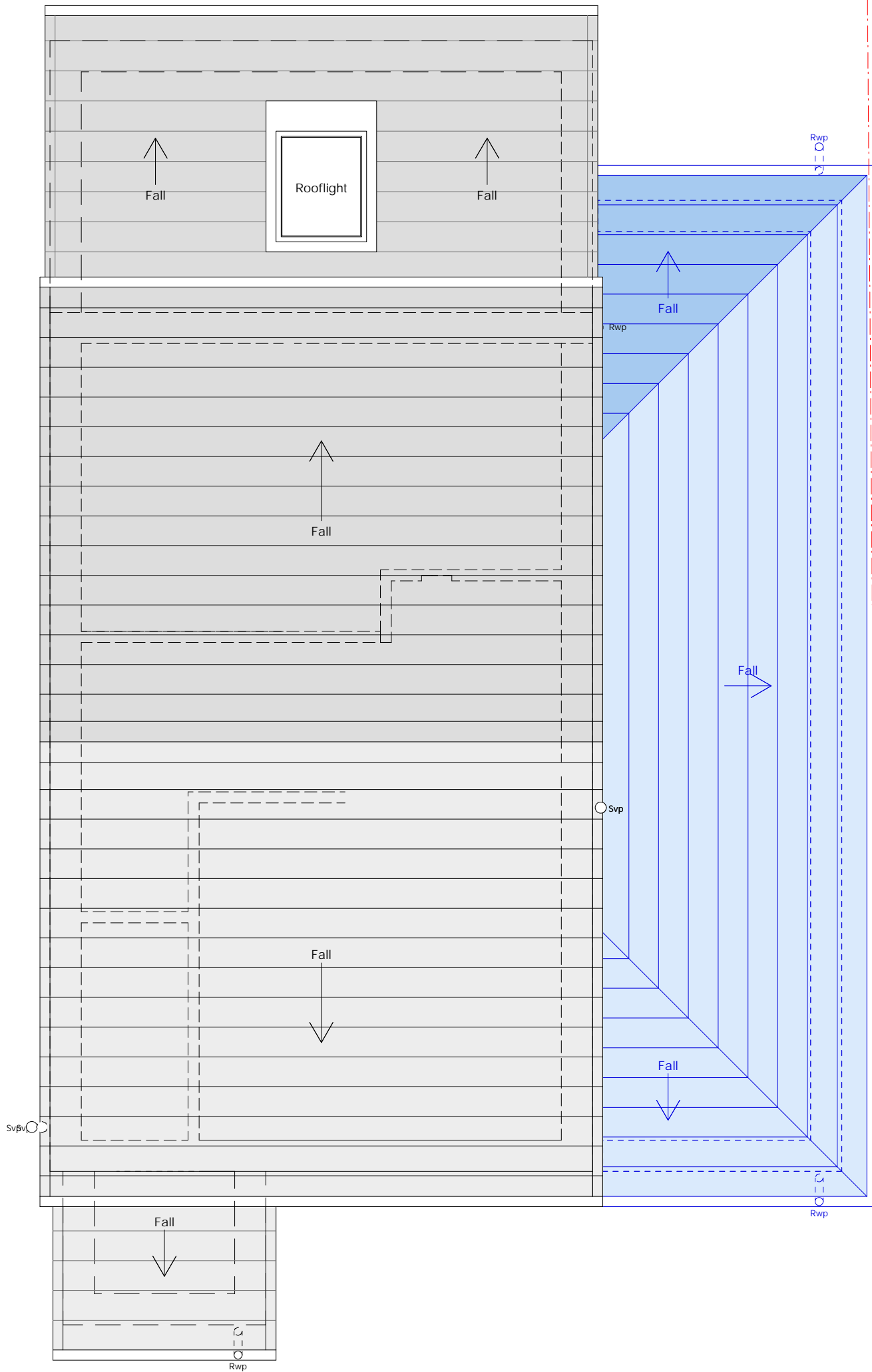
Roof Plan as Proposed Scale 1:50@A3
