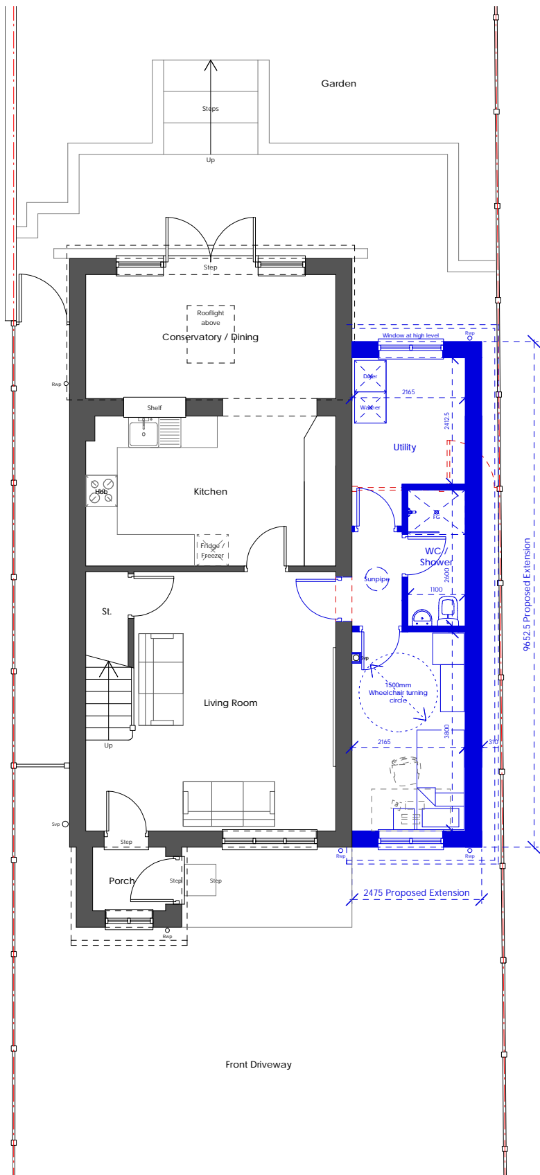
Ground Floor Plan as Proposed Scale 1:100@A3
