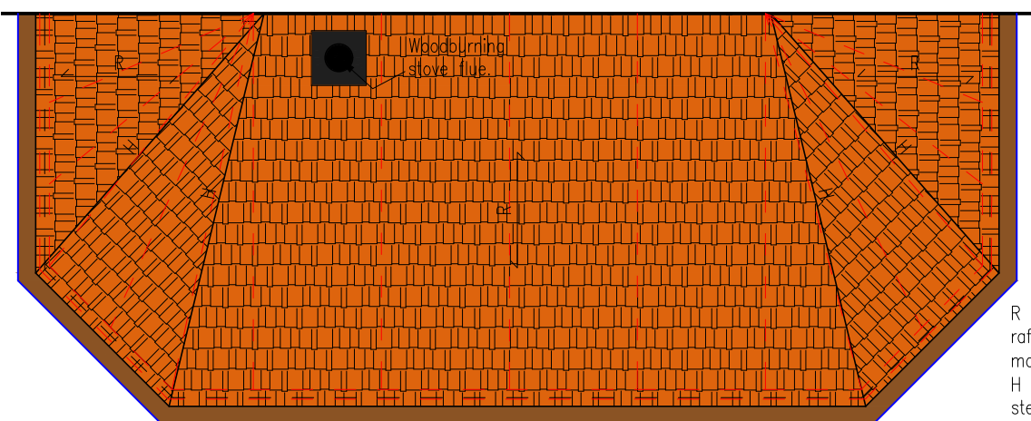
Proposed Roof Plan 1: 50
