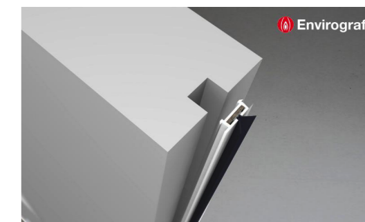
Recessed fire strip with smoke seal
