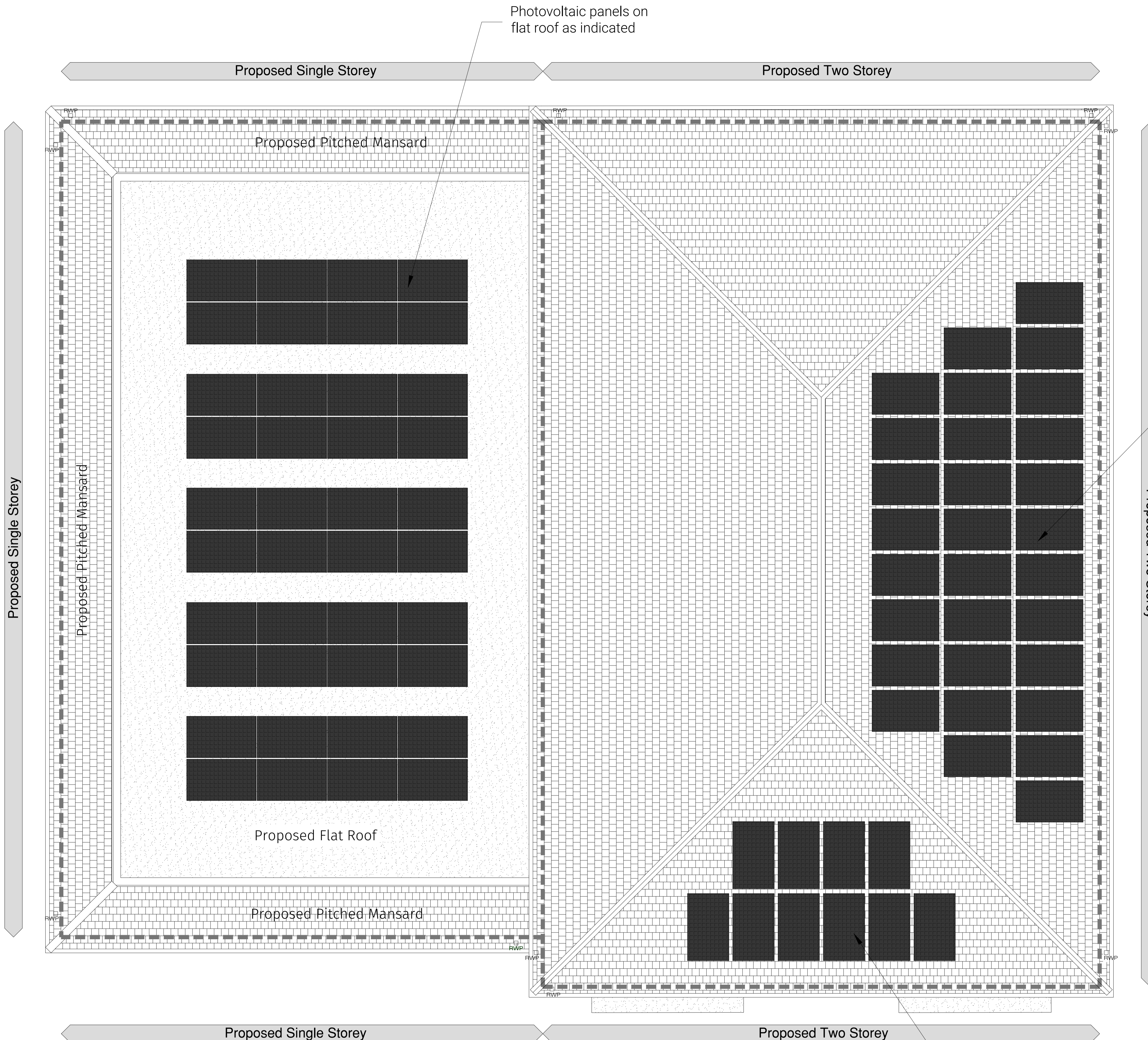
1 PROPOSED ROOF PLAN 1:50
