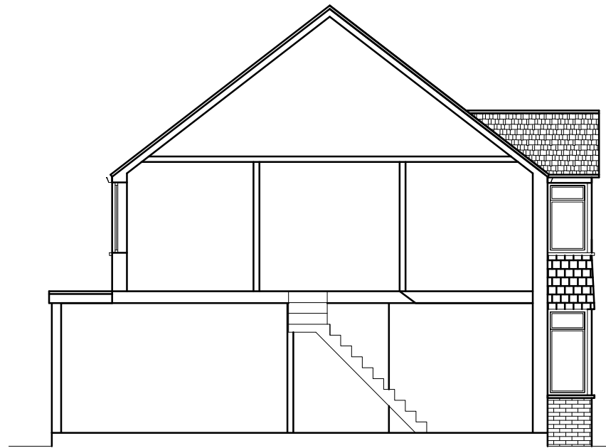
EXISTING SECTION
