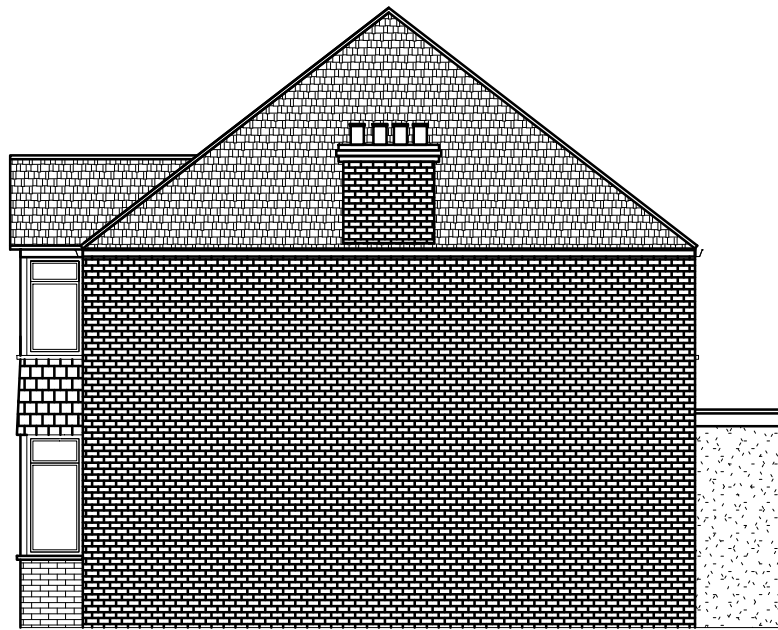
EXISTING RIGHT SIDE ELEVATION
