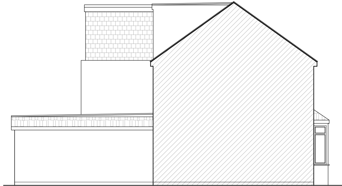
Existing / Proposed Left Side Elevation
