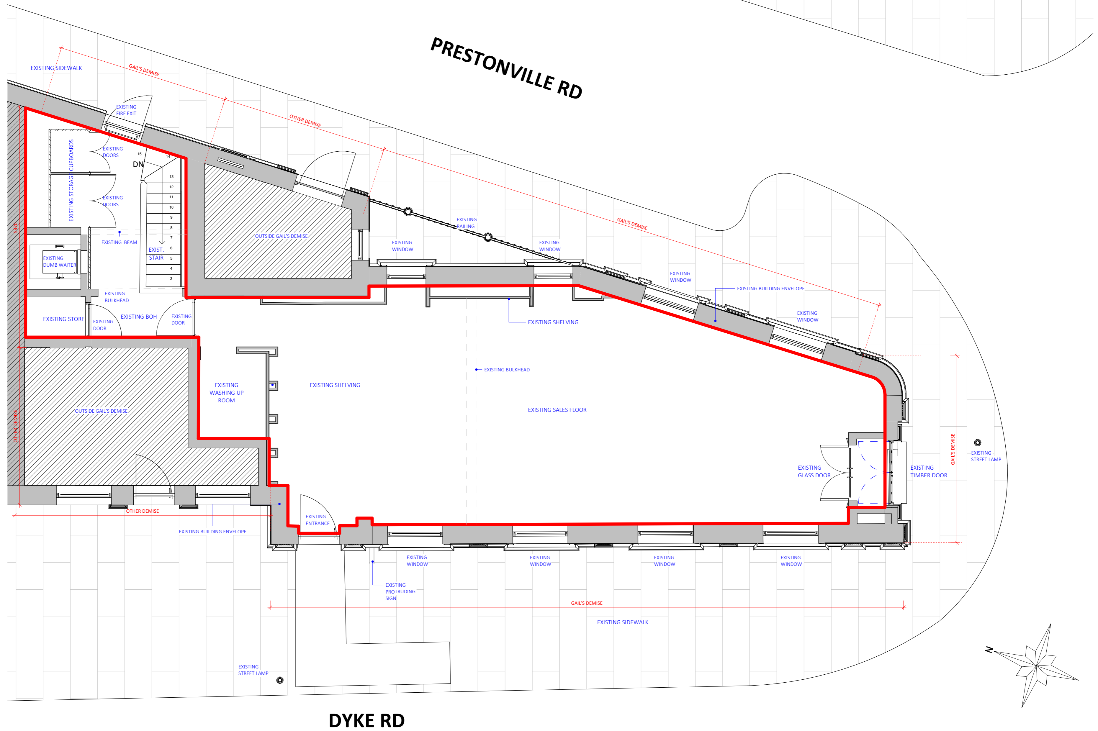
Ground Floor - Existing_AA scale 1 : 50
