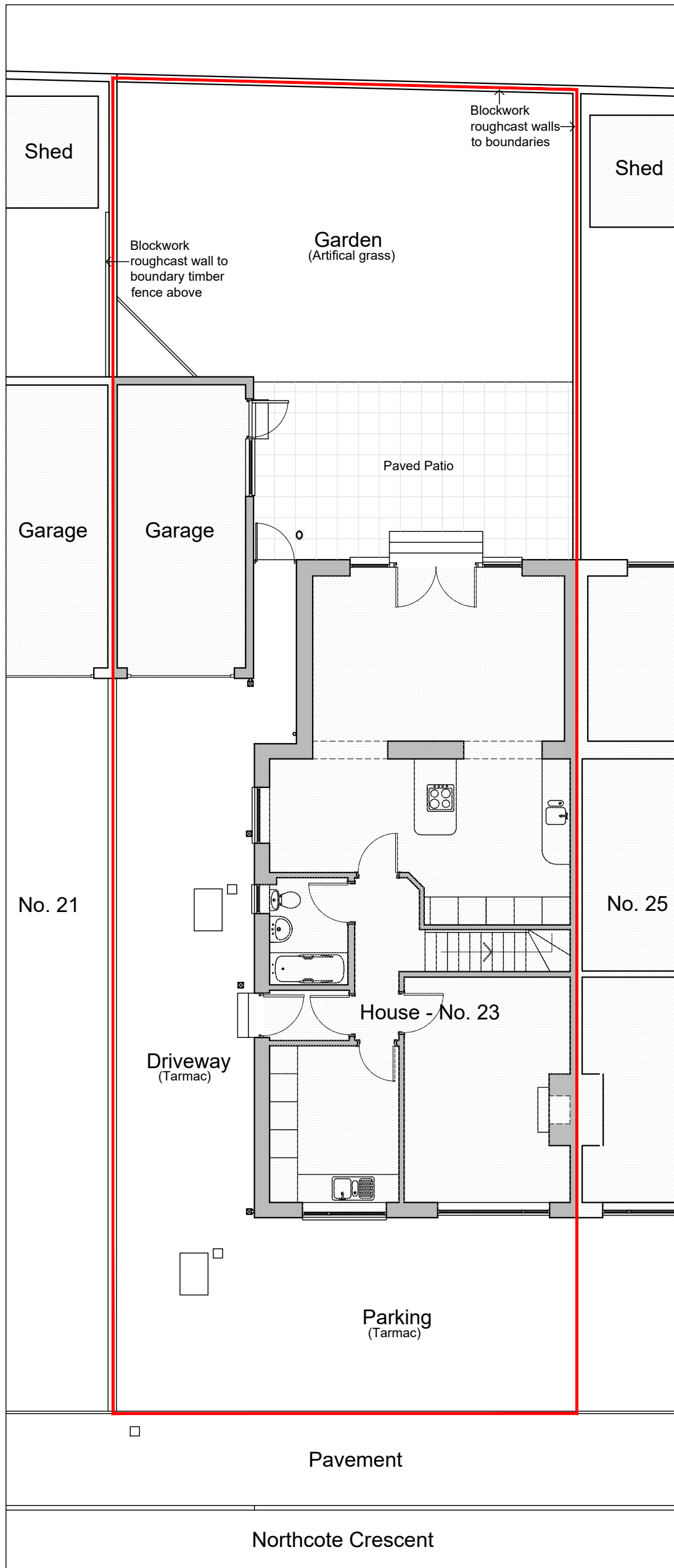
Existing Site Plan 1:100 @ A3
