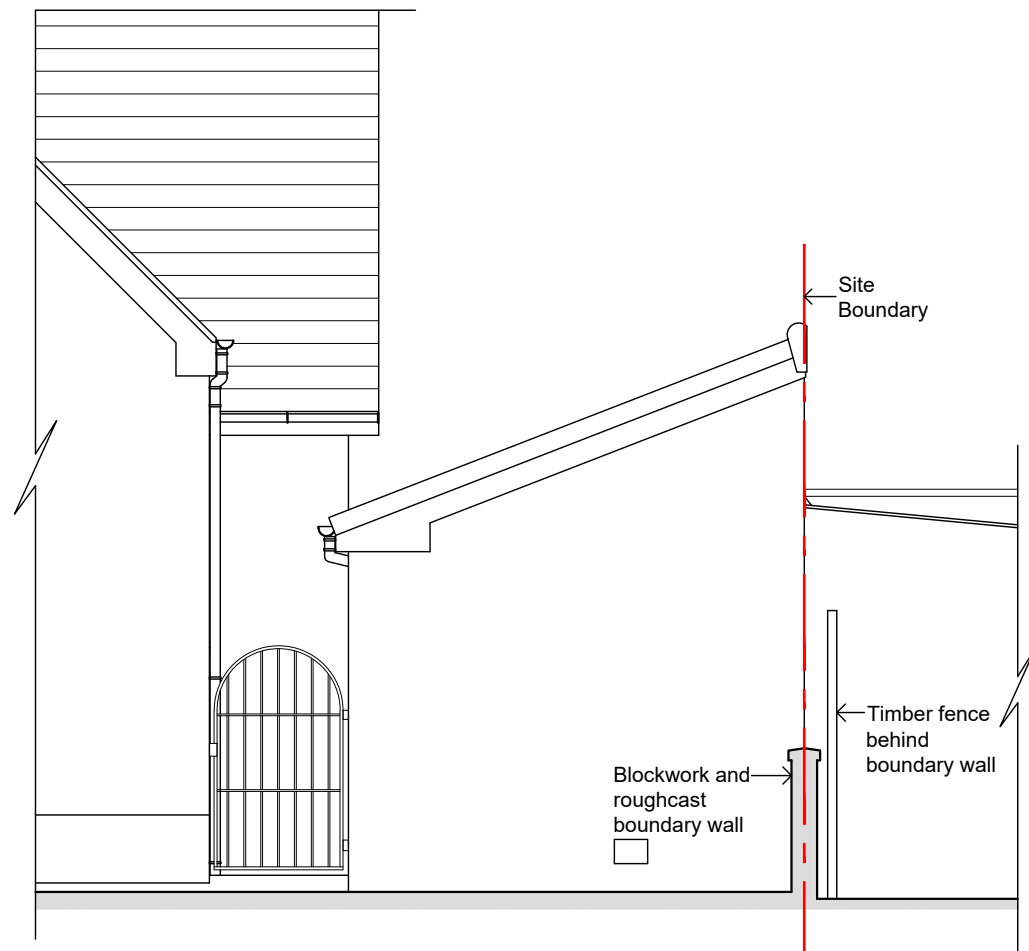
North East Elevation (Looking to Garage)
