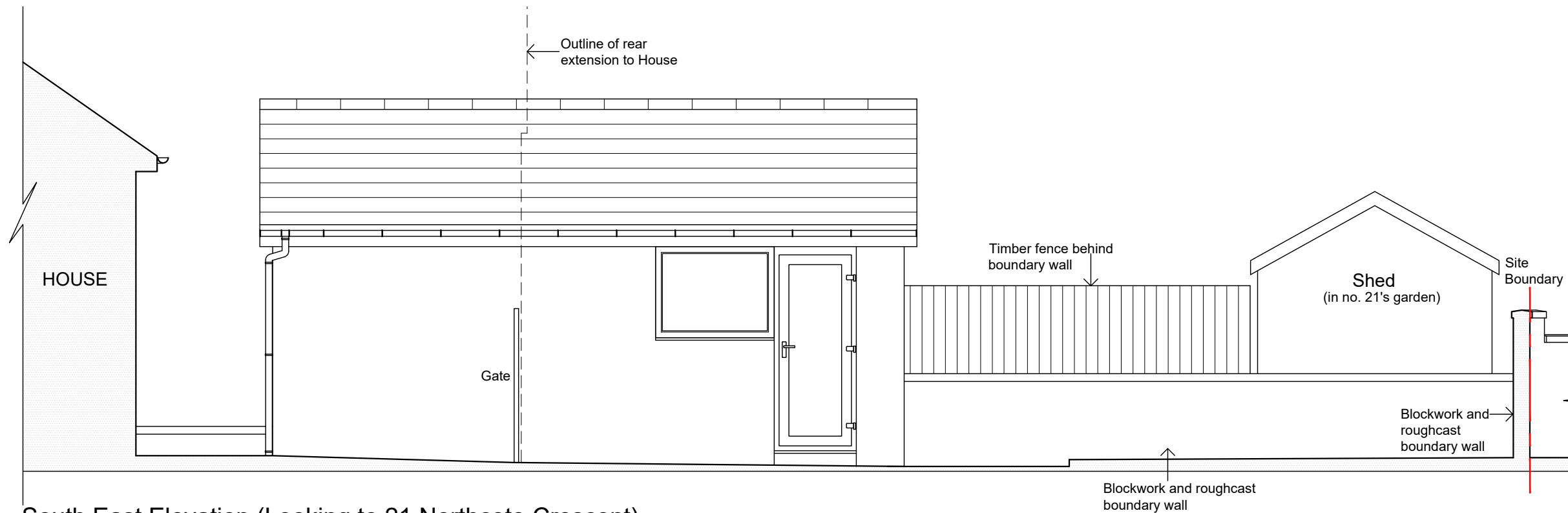
South East Elevation (Looking to 21 Northcote Crescent)
