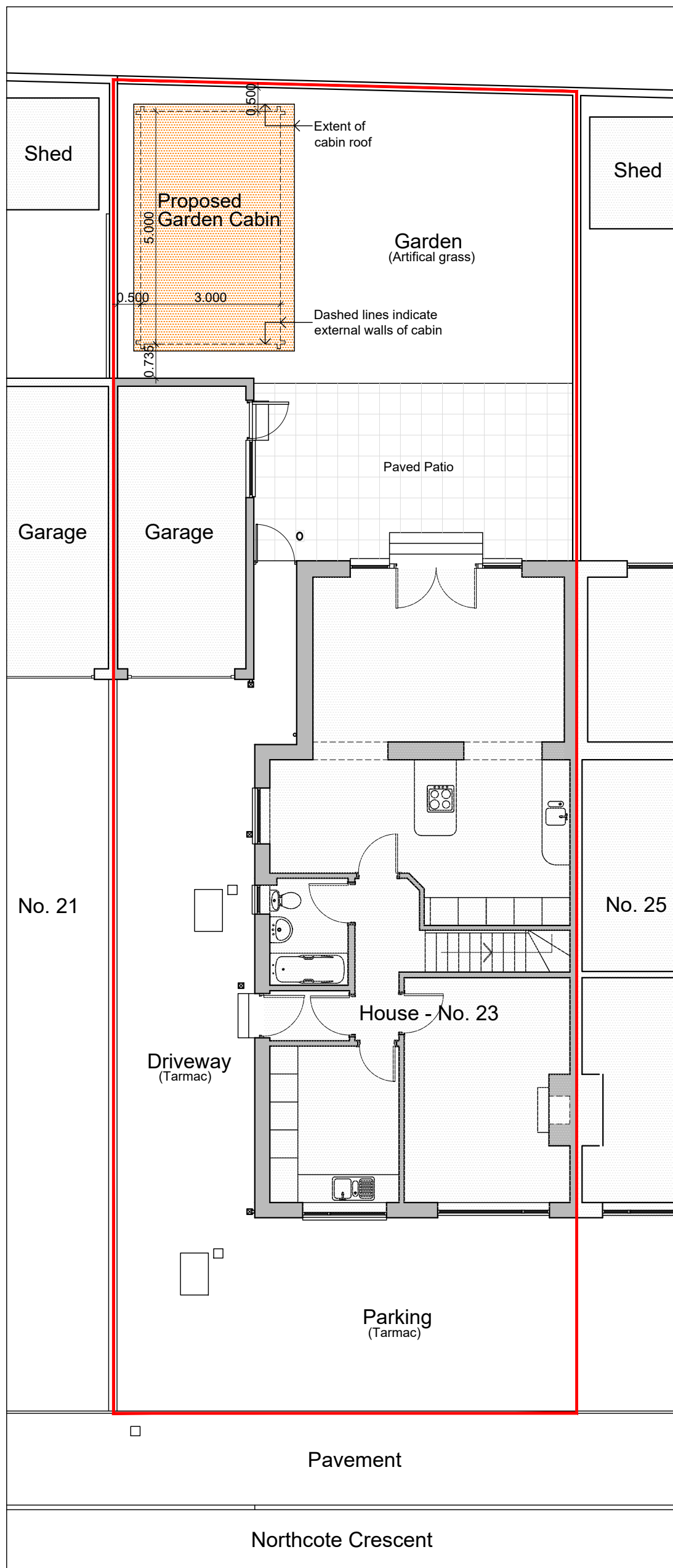
Proposed Site Plan 1:100 @ A3
