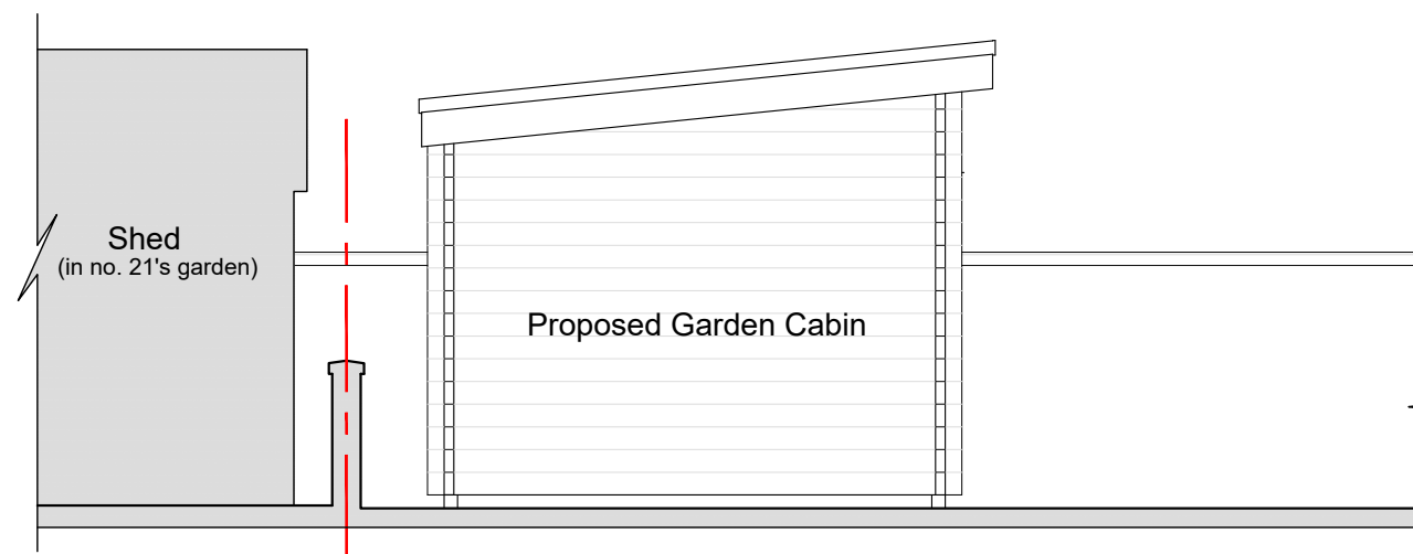
South West Elevation (Looking to Rear Boundary)
