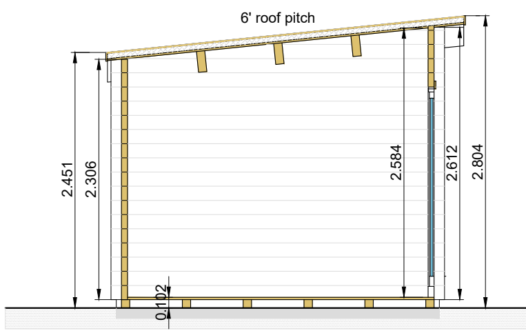
Section A-A Cabin Plan, Elevations & Section
