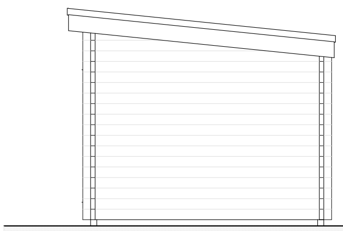
Side (South West) Elevation
