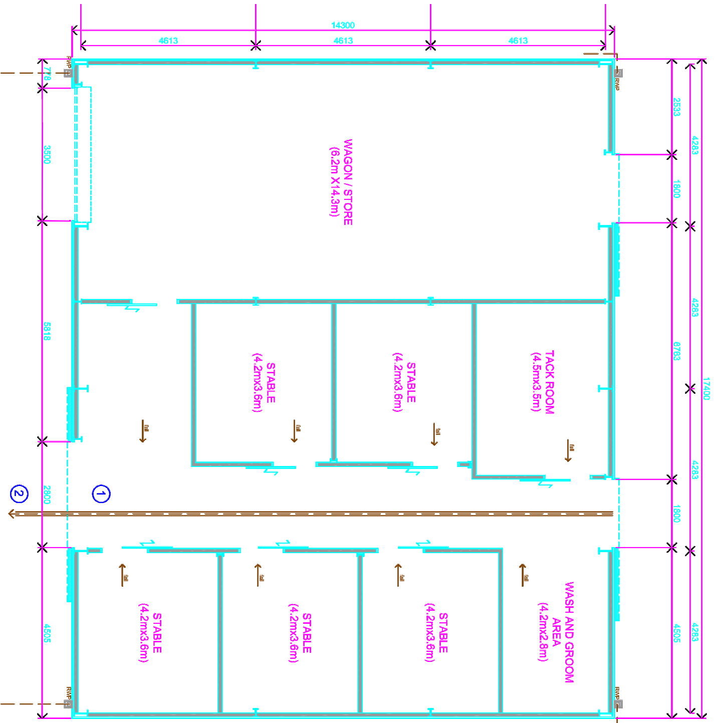
Proposed Floor Plan - 1:100
