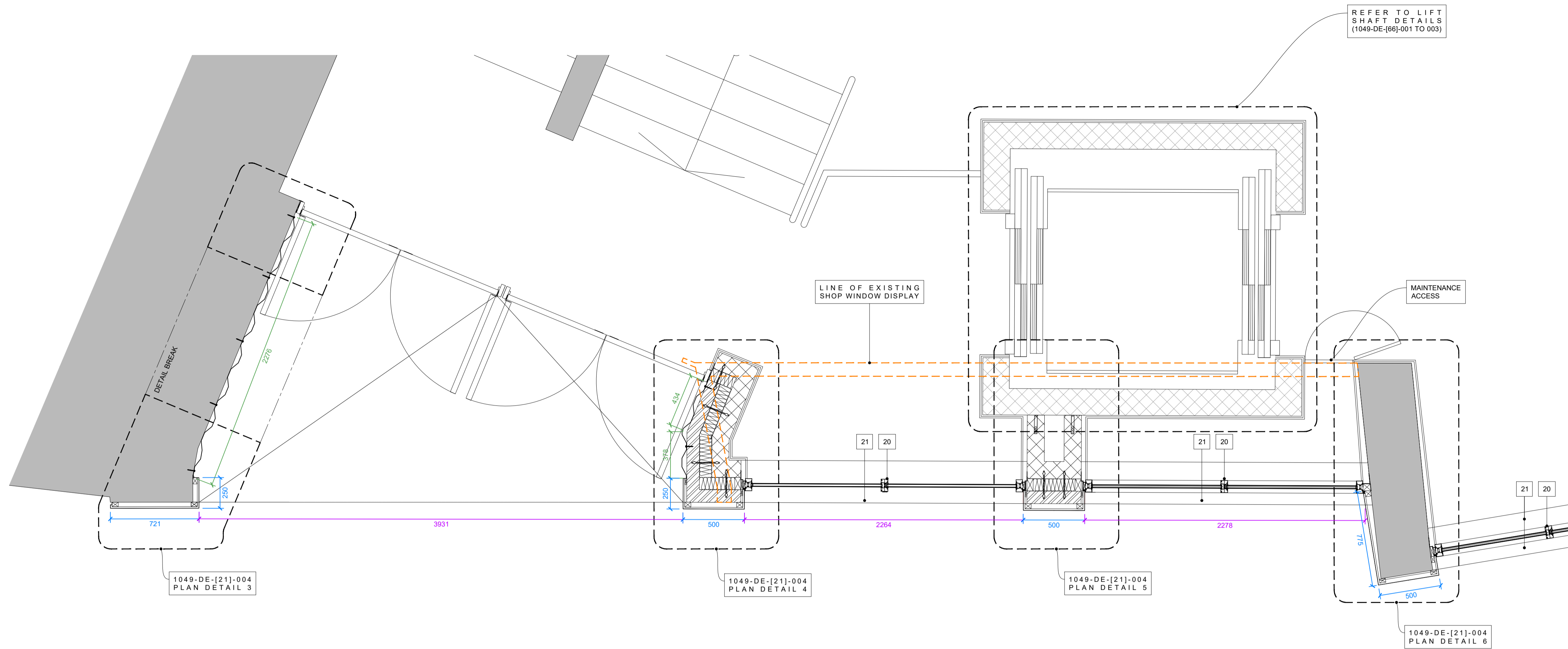
1049-DE-[21]-002 - PLAN DETAIL 01 SCALE 1:20
