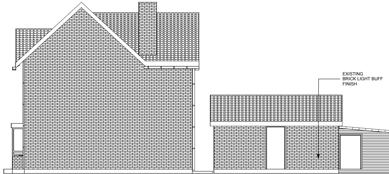
SIDE ELEVATION 1:100
