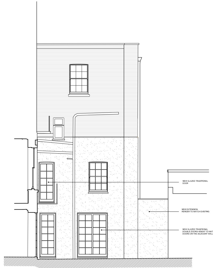
SIDE ELEVATION - APPROVED UNDER APPLICATION 22/07938/FULL
