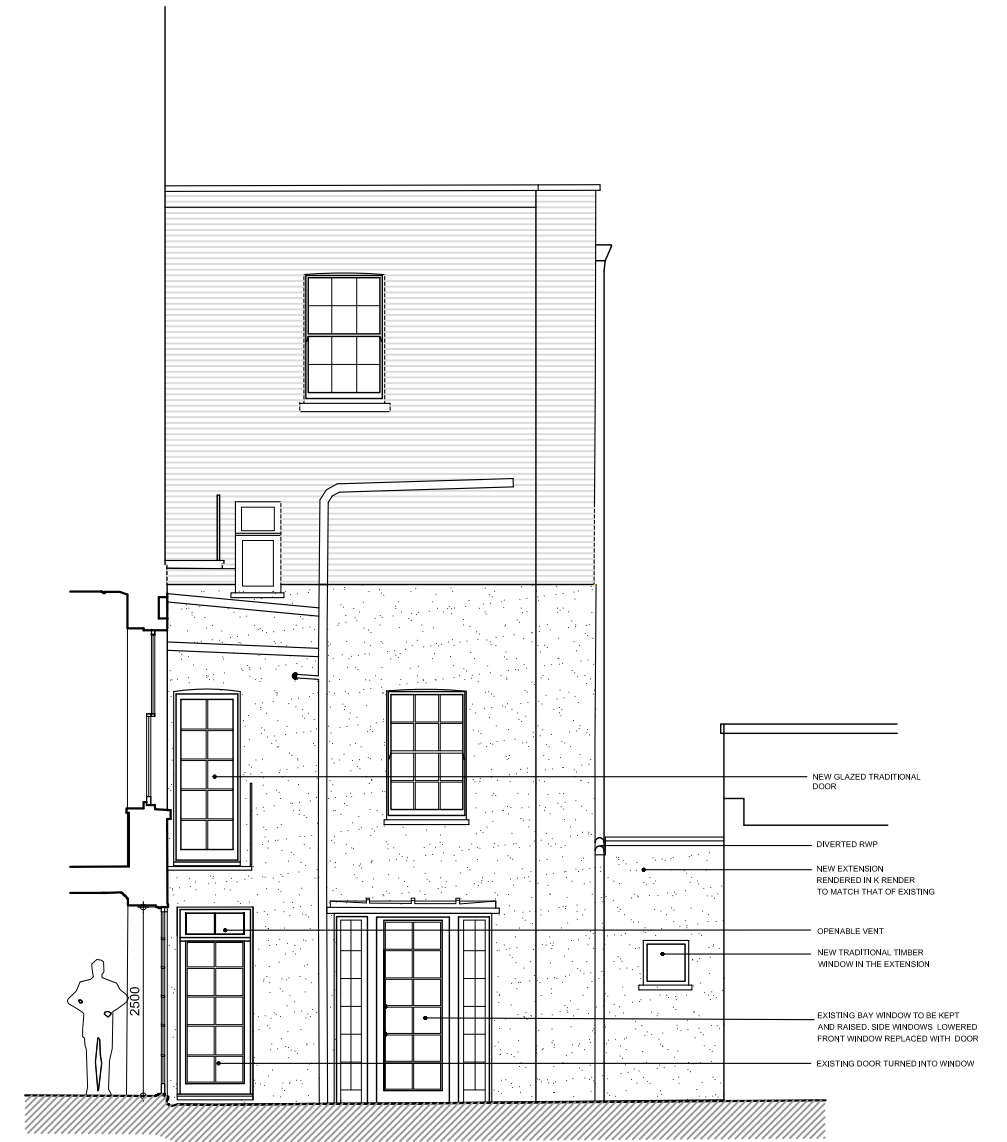
SIDE ELEVATION - Proposed
