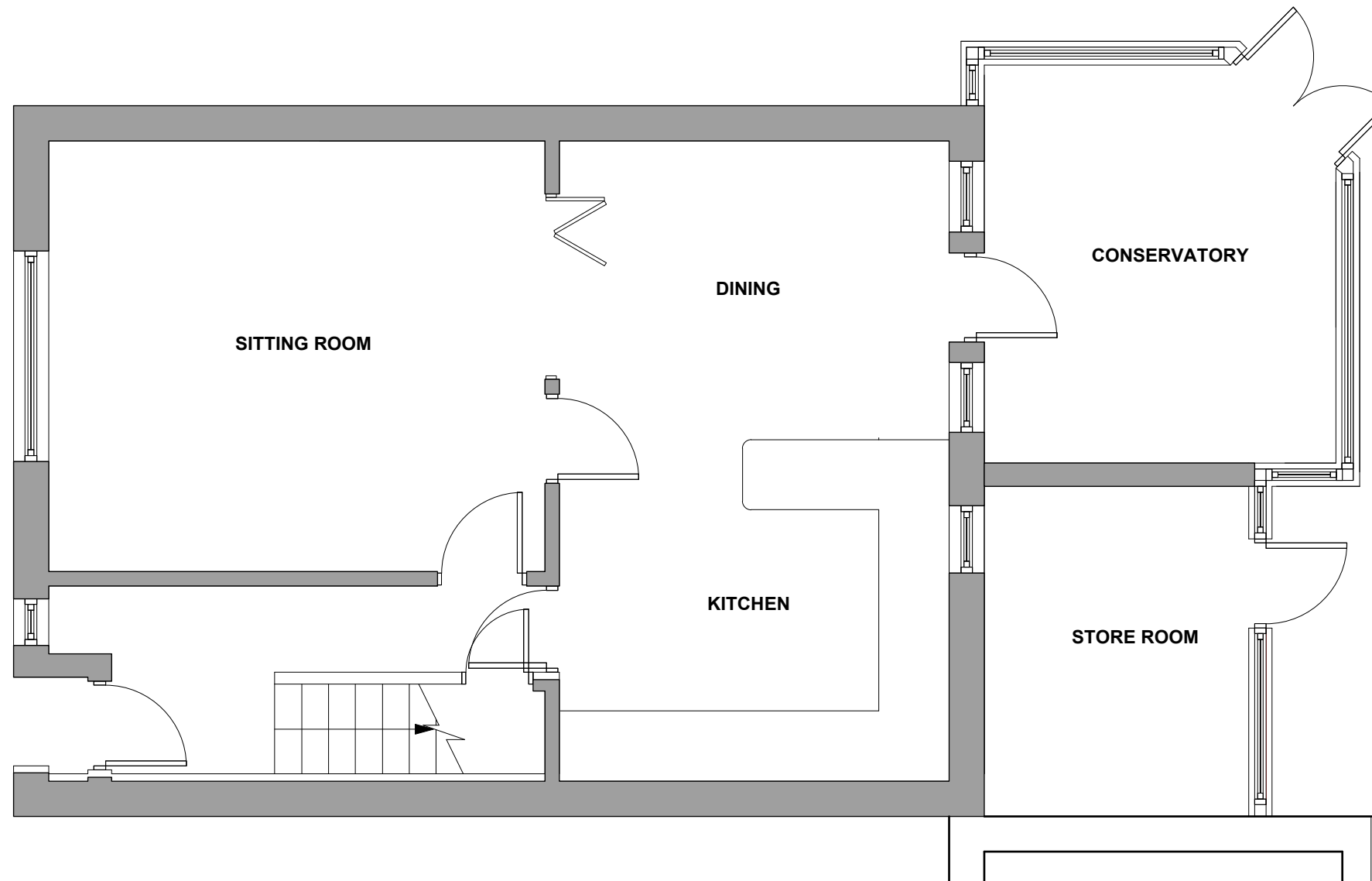
EX01 Existing Ground Floor 1:50 @ A3
