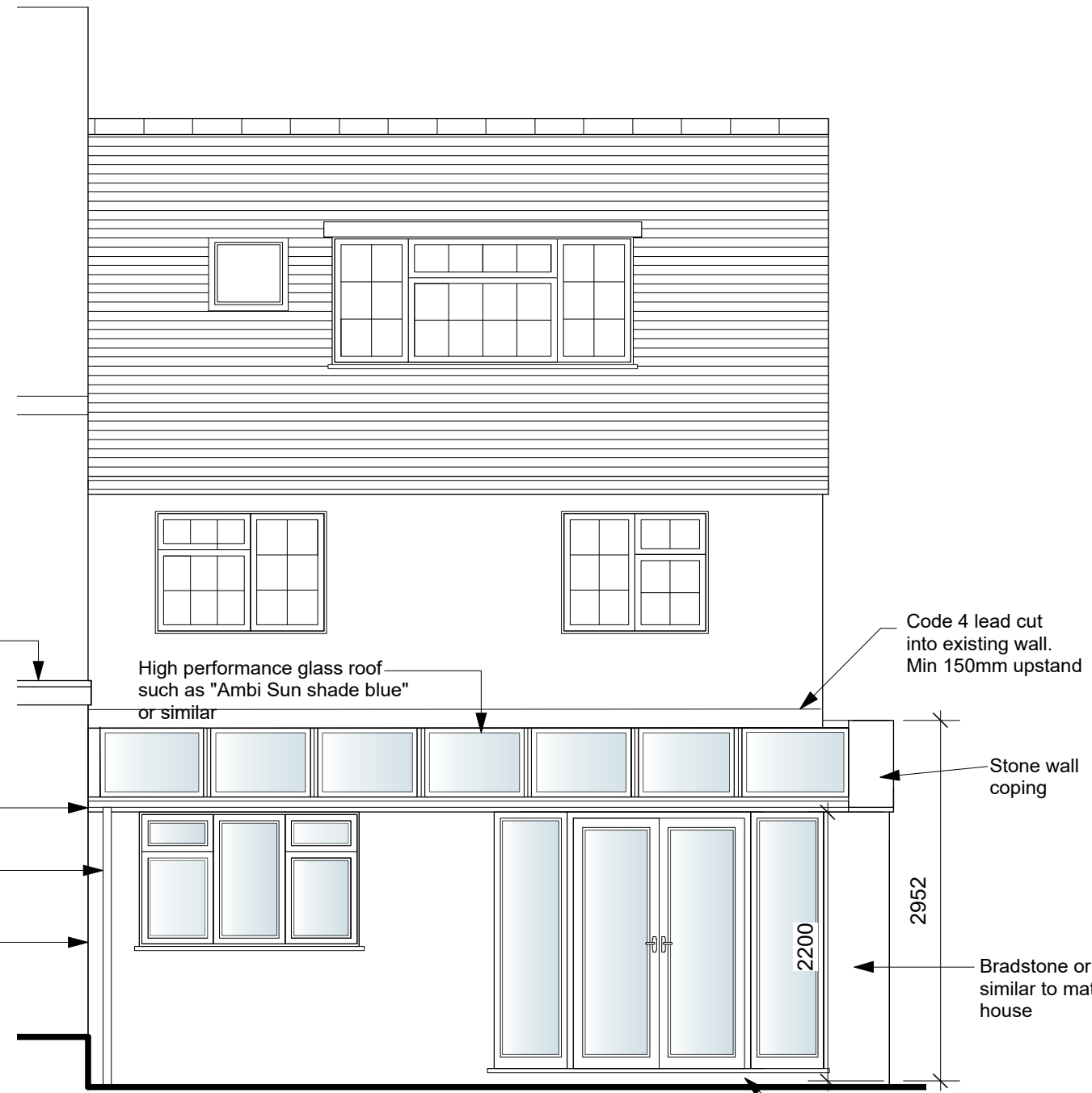
PR02 Proposed Rear Elevation 1:50 @ A3
