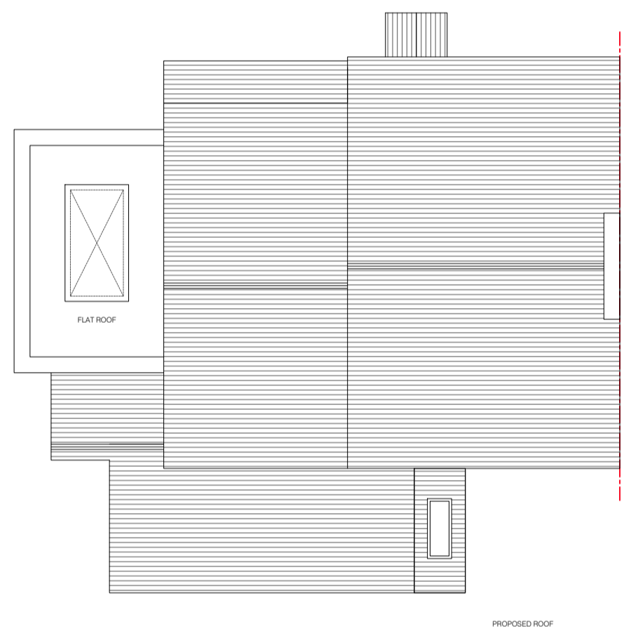
PROPOSED ROOF
