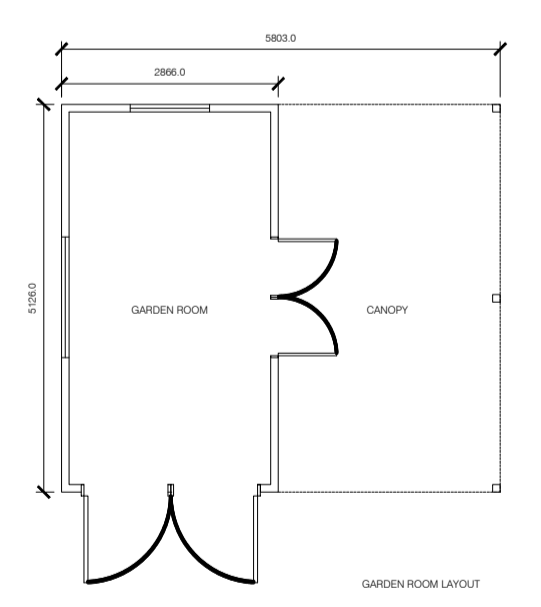
GARDEN ROOM LAYOUT
