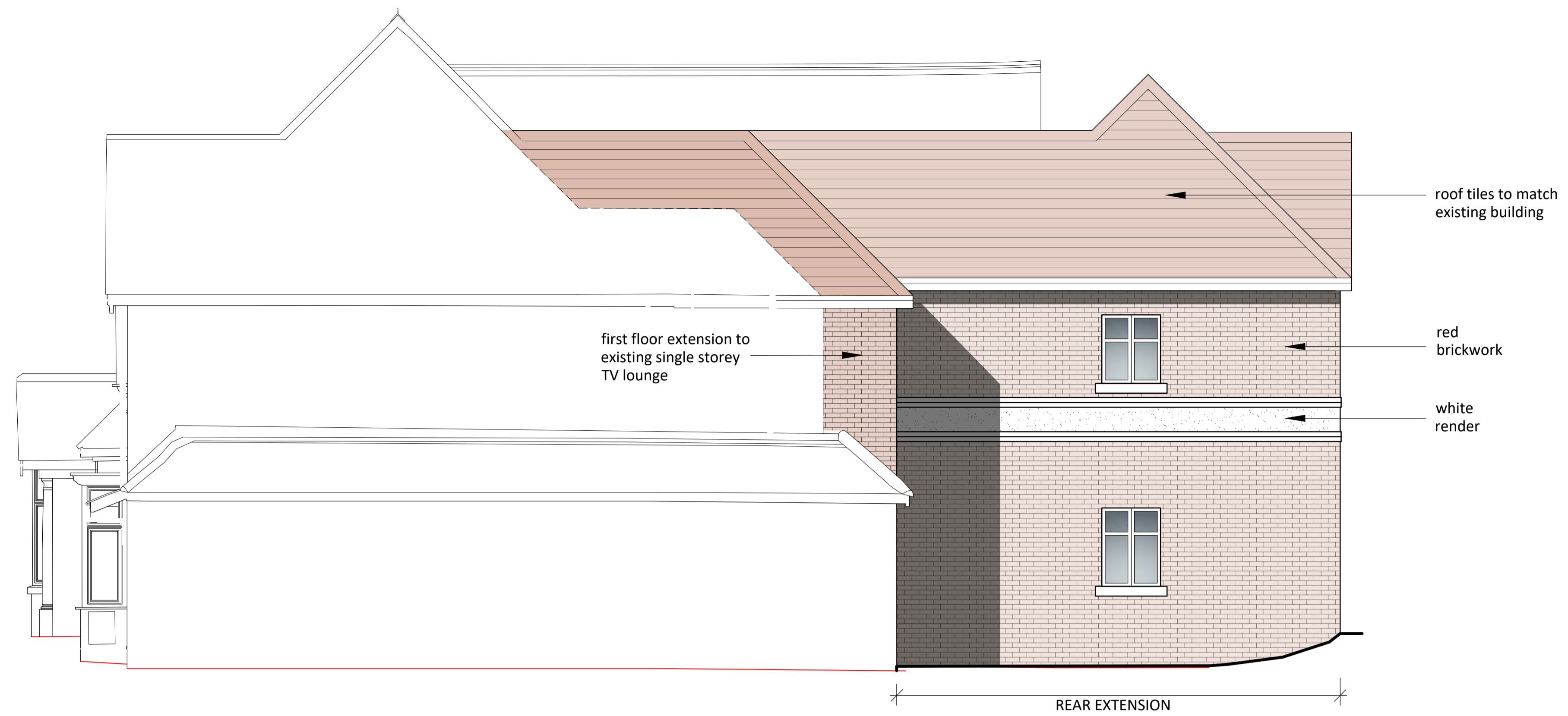
SIDE ELEVATION - NORTH
