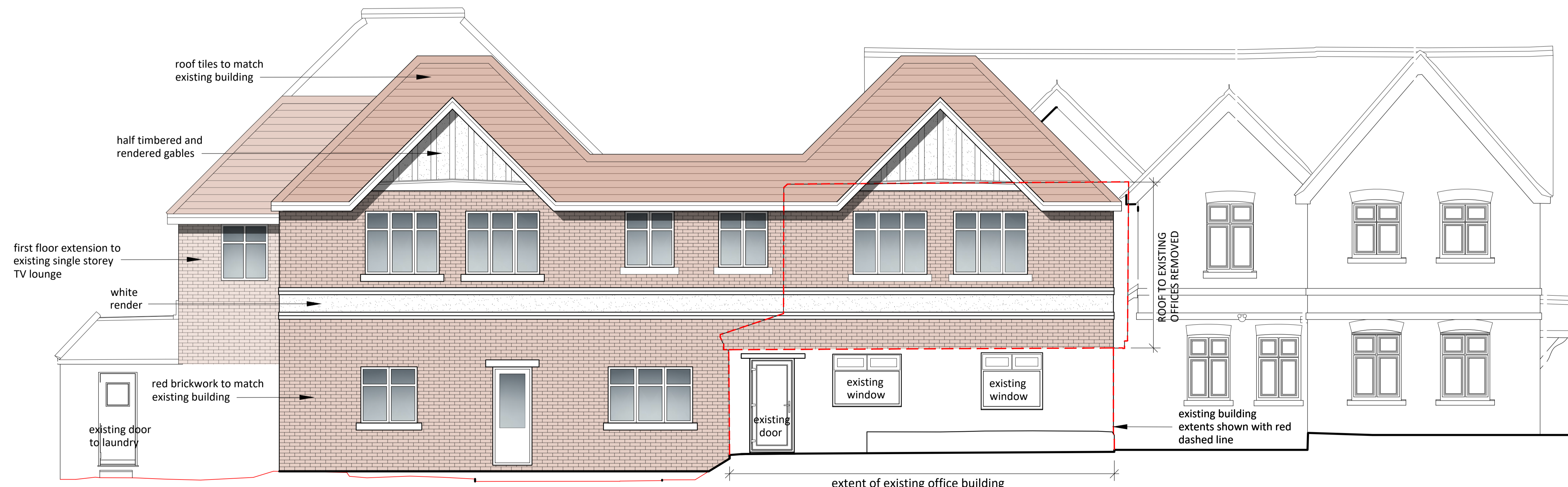
REAR ELEVATION
