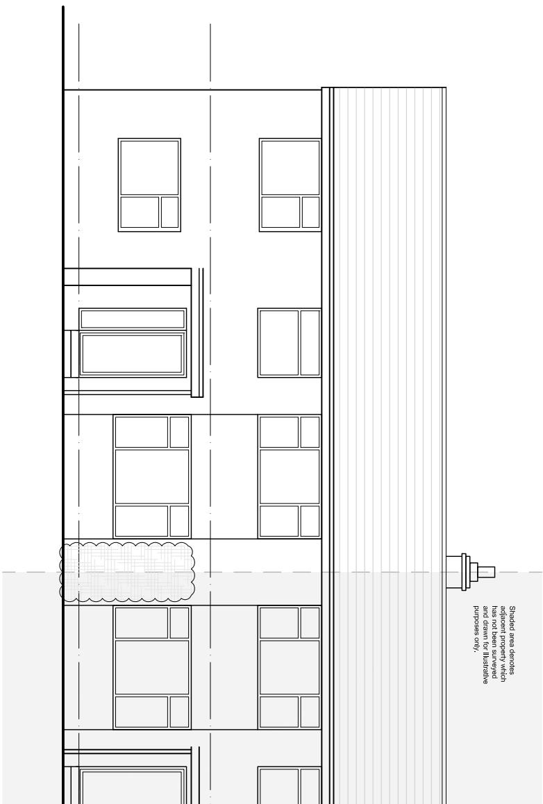
North West (Front and Principal) Elevation
