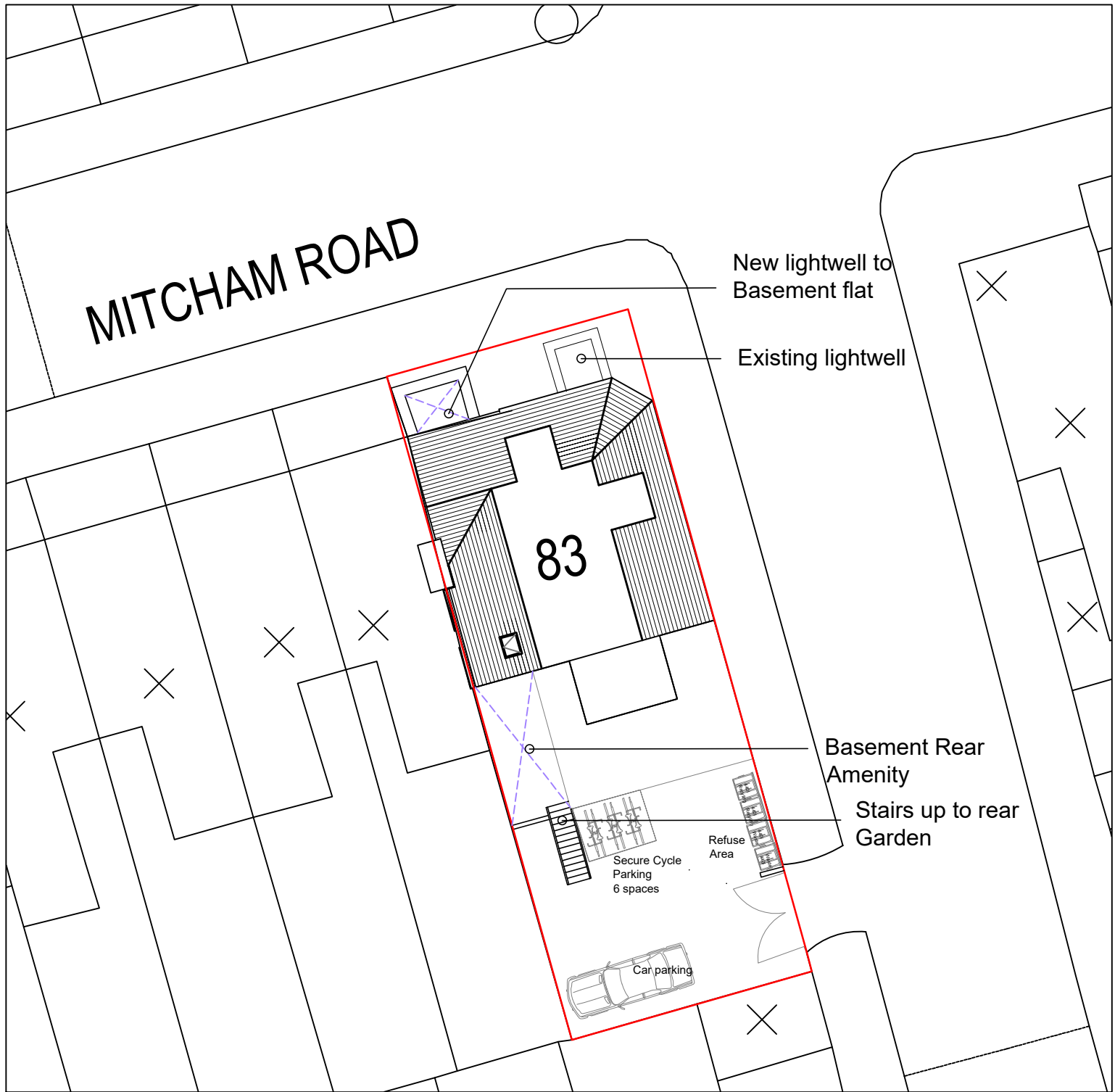
Block Plan
