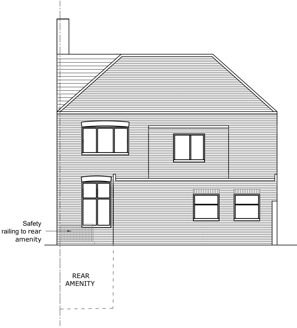
Proposed Rear Elevation 1:100
