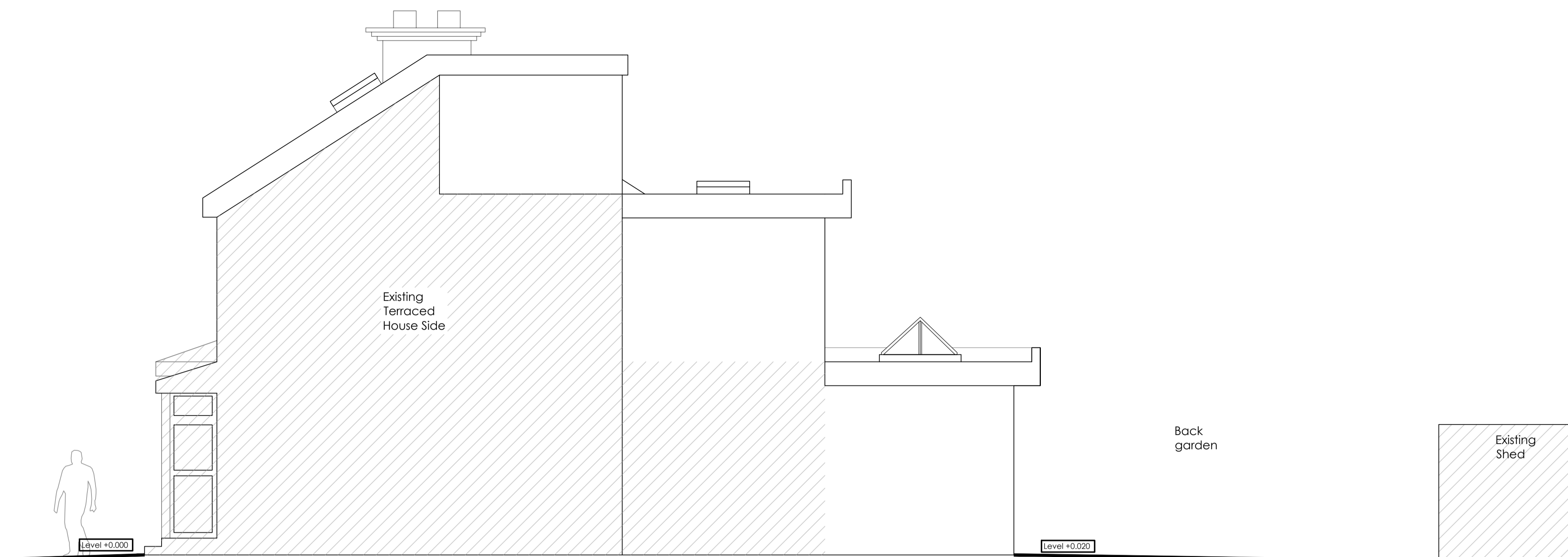
Proposed side Elevation (South East) Scale 1:50@A1
