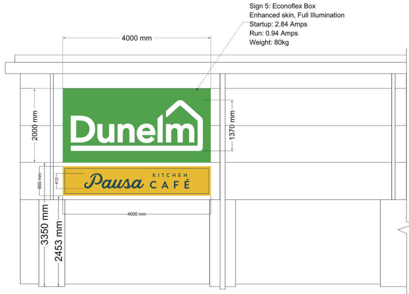
REAR ELEVATION
