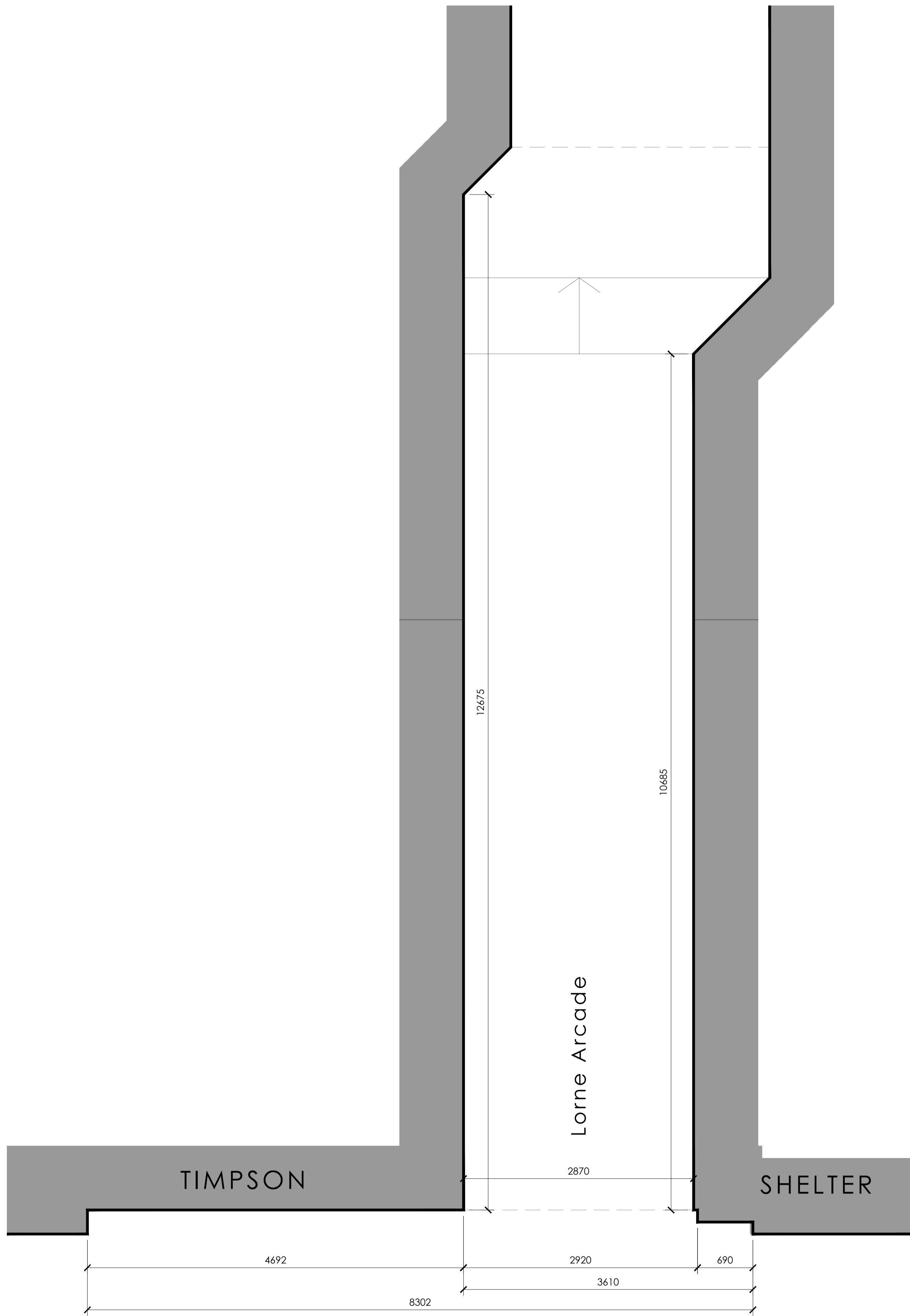
EXISTING - EAST (HIGH STREET) PLAN 1:50
