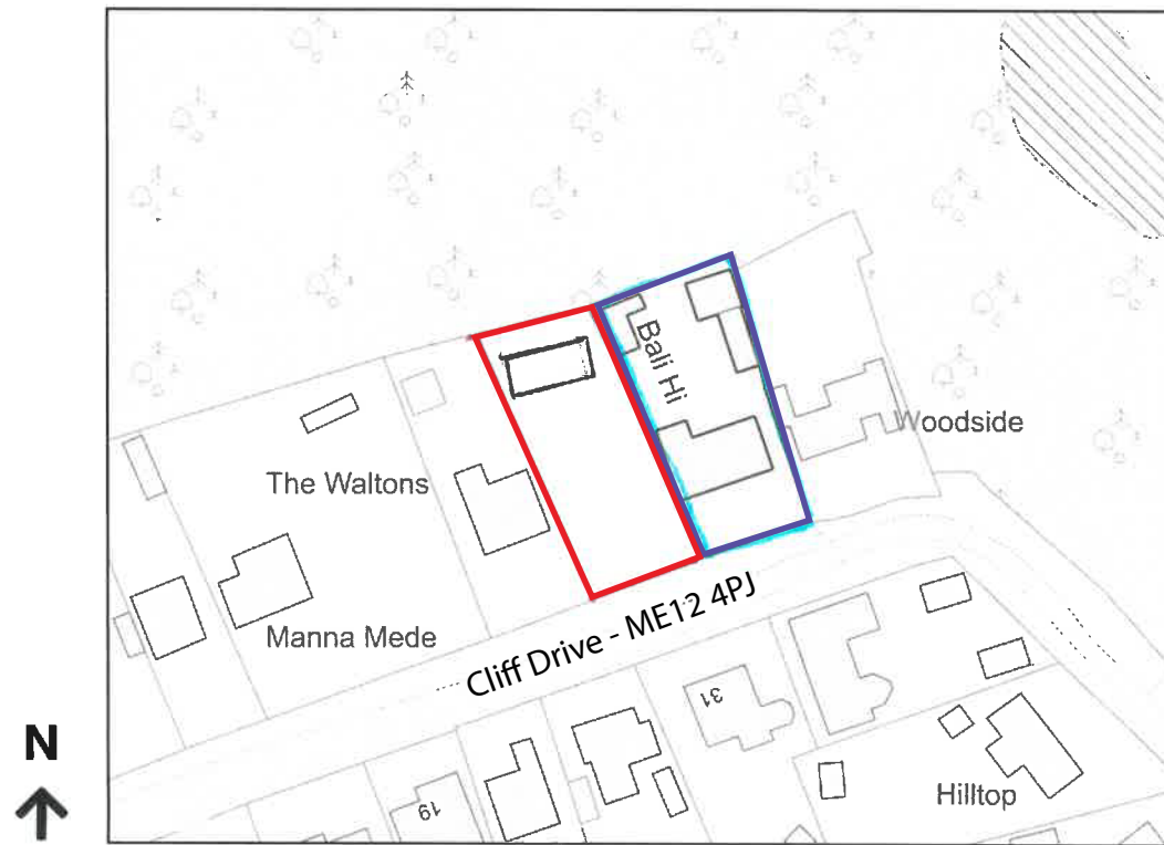
Block and Site plan showing Shed/garage/caravan store as part built
