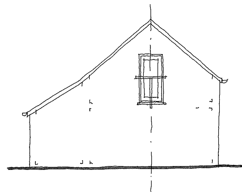
EAST ELEVATION GARAGE 1:100 @ A3
