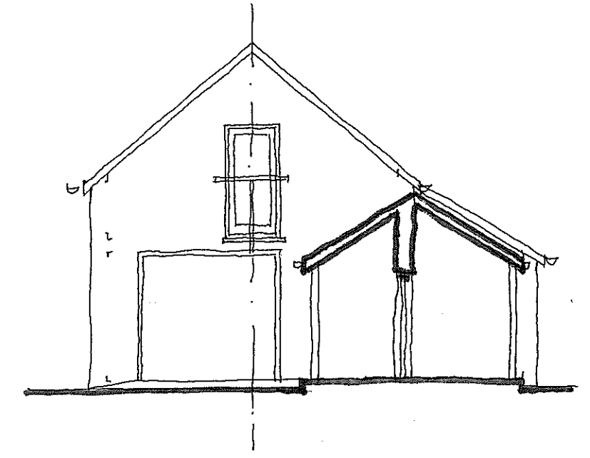
WEST ELEVATION GARAGE. 1:100 @ A3
