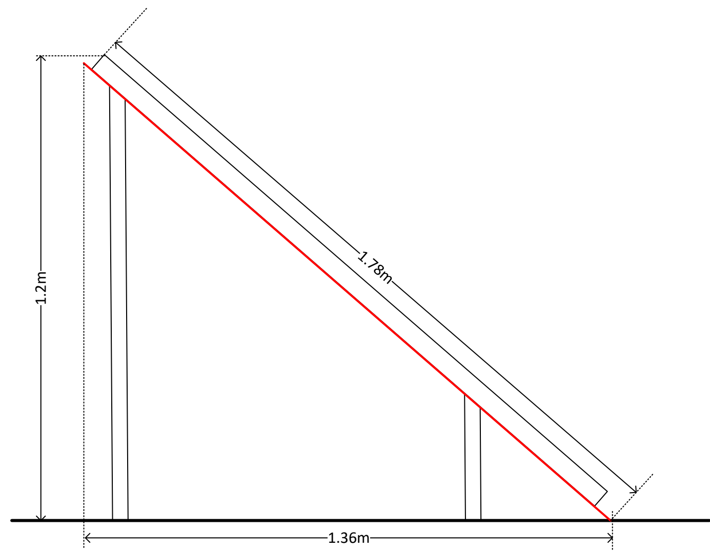
Side View
