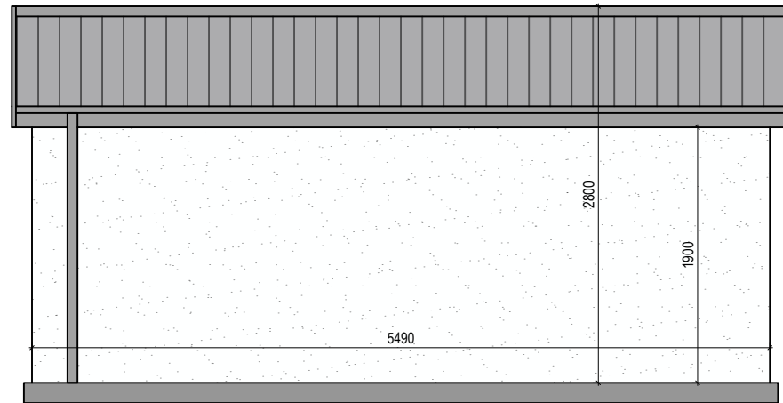
PROPOSED NORTH ELEVATION SCALE 1:50
