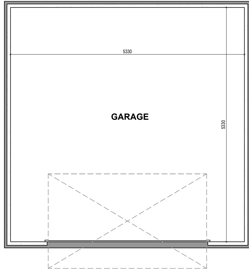
PROPOSED FLOOR PLAN SCALE 1:50
