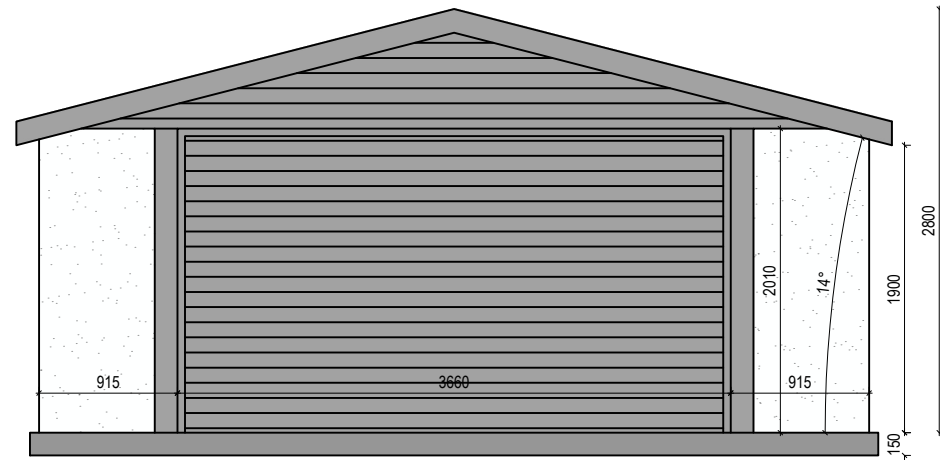
PROPOSED WEST ELEVATION SCALE 1:50
